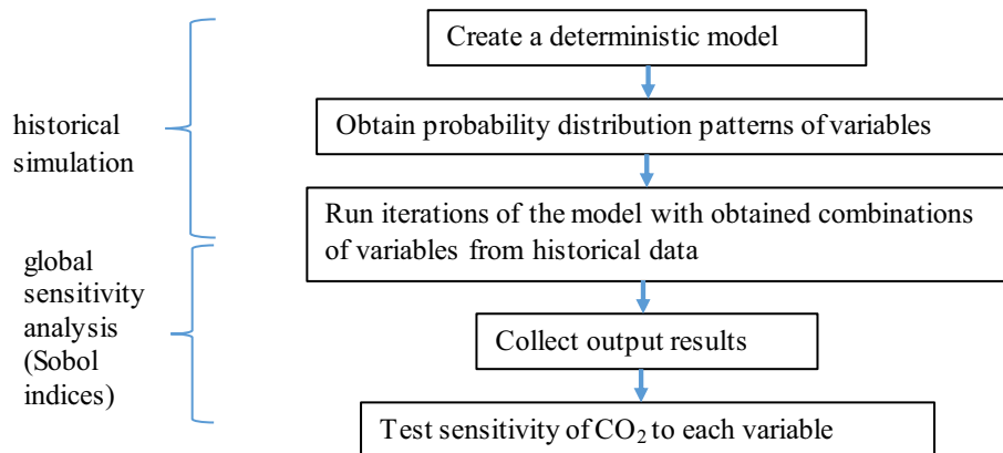
Fig. 3. Methodology.
