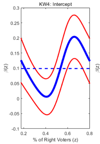
Figure 2: Estimates coefficient function of the intercept: Z represents vote
