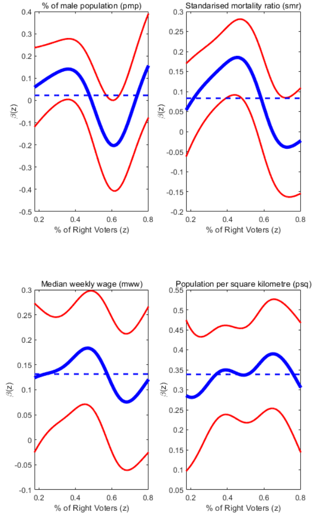
Figure 3: Estimates coefficient functions based on KW4: Z represents vote
