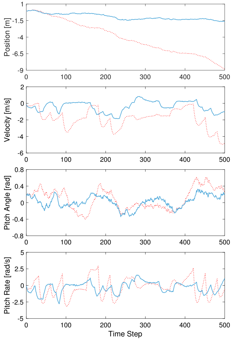
FIGURE 3. The position, velocity, pitch angle, and pitch rate trajectories. The solid lines represent the trajectories under the triggering policy designed based on the value of information, and the dotted lines represent the trajectories under a periodic triggering policy.
