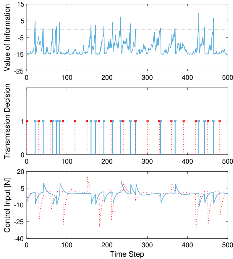
FIGURE 2. The value of information, transmission decision, and control input trajectories. The value of information is scaled by one tenth. The solid lines represent the trajectories under the triggering policy designed based on the value of information, and the dotted lines represent the trajectories under a periodic triggering policy.
