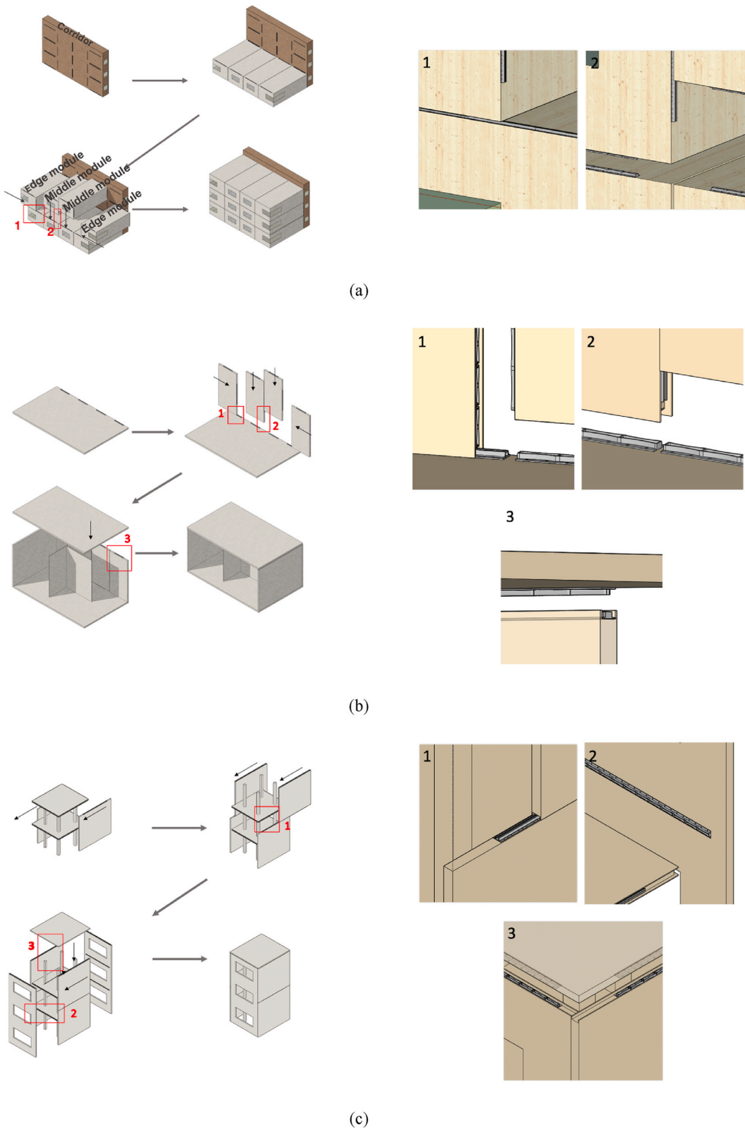
Fig. 4. Application overview of the novel interlocking connection system for different CLT modular structures and the close-up of construction details: (a) CLT volumetric structures (b) CLT panelised platform-type structures (c) CLT panelised balloon-type structures.
