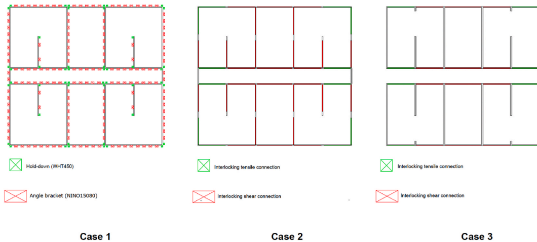
Fig. 18. Interlocking connection locations in different buildings.
