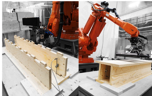
Fig. 13. Robotic assembly of a box girder with through-tenon joints [49].
