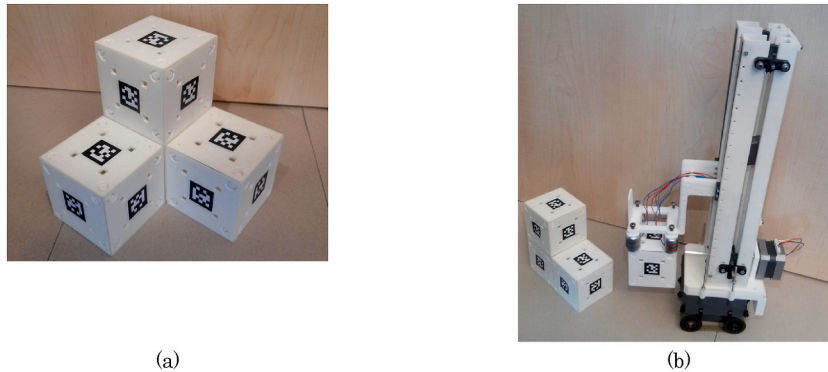
Fig. 10. Prototypes of (a) the stigmergic building block and (b) the mobile robot [45].
