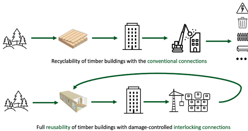
Fig. 8. Comparison of potential building life cycles between CLT structures utilising conventional connections (top) and MOD-IT connections (bottom).
