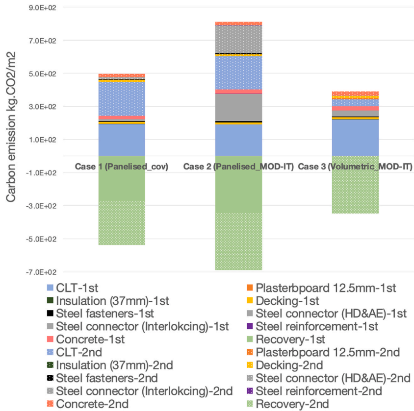
Fig. 17. Contribution of different building components to the carbon emission.
