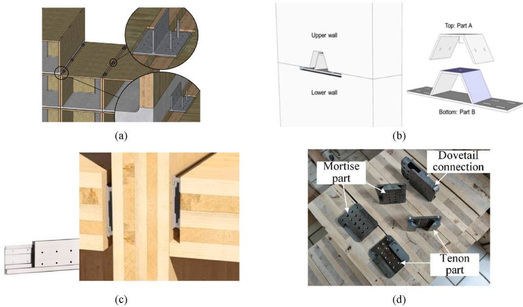
Fig. 3. Novel interlocking metal connections for modular CLT structures: (a) Connection for Jakarta Hotel project [36] (b) An inter-module horizontal connection proposed by the University of British Columbia [37] (c) LOCK Connector from Rothoblaas Ltd [38]. (d) Prefabricated metal dovetail connector [39].
