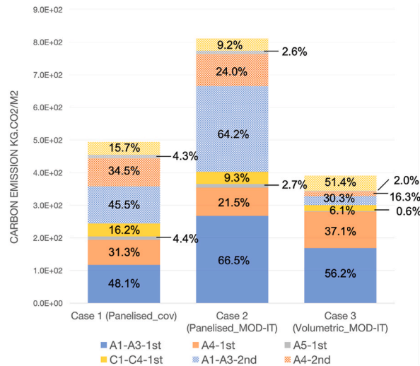
Fig. 19. Relative contributions of the building's life cycle stages to the environmental impacts (Note: The above percentages refer to the proportion of each stage within their respective building life cycles.).
