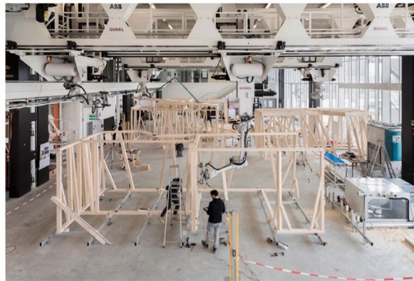
Fig. 11. The assembly of the DFABHOUSE [46].
