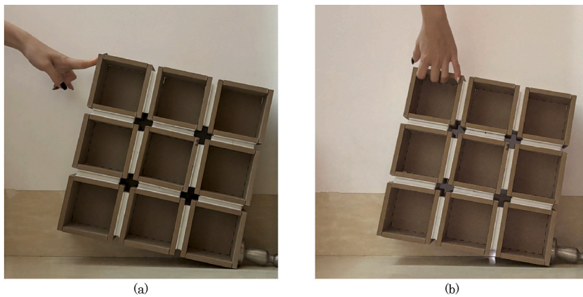
Fig. 7. Interlocking connection-reinforced timber modules under (a) lateral and (b) vertical load.
