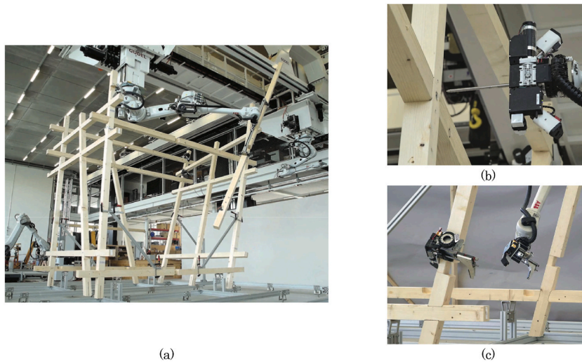
Fig. 12. Construction of CantiBox: (a) timber units during construction with the robotic arm; (b) robotic screwdriver on key components; (c) interlocking connections in the structures assembled by the robotic arm [48].
