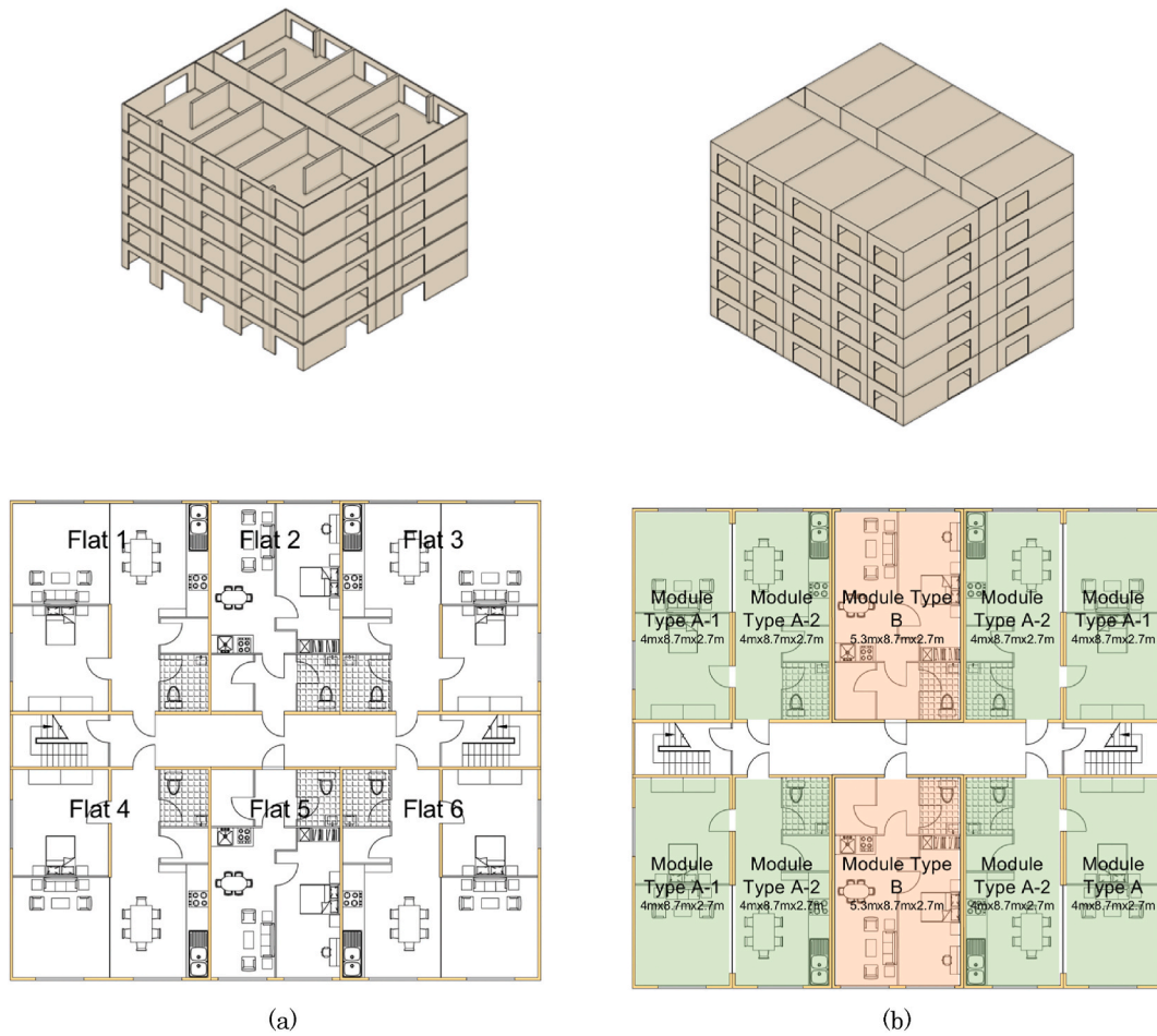
Fig. 14. Floor plans and overall structure of the (a) panelised building and (b) the volumetric buildings.
