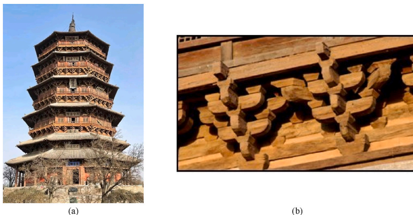
Fig. 1. The tallest and oldest existing timber tower in China (a) Yingxian wooden pagoda, first built in 1056AD, and (b) its interlocking connection details [9].
