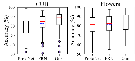
Figure 5. The boxplots of the test classification accuracies of ProtoNet, FRN and our method (Ours) across 100 randomly sampled tasks. The models are trained by the 10-way 5-shot setting and evaluated by 5-way 1-shot test tasks.
