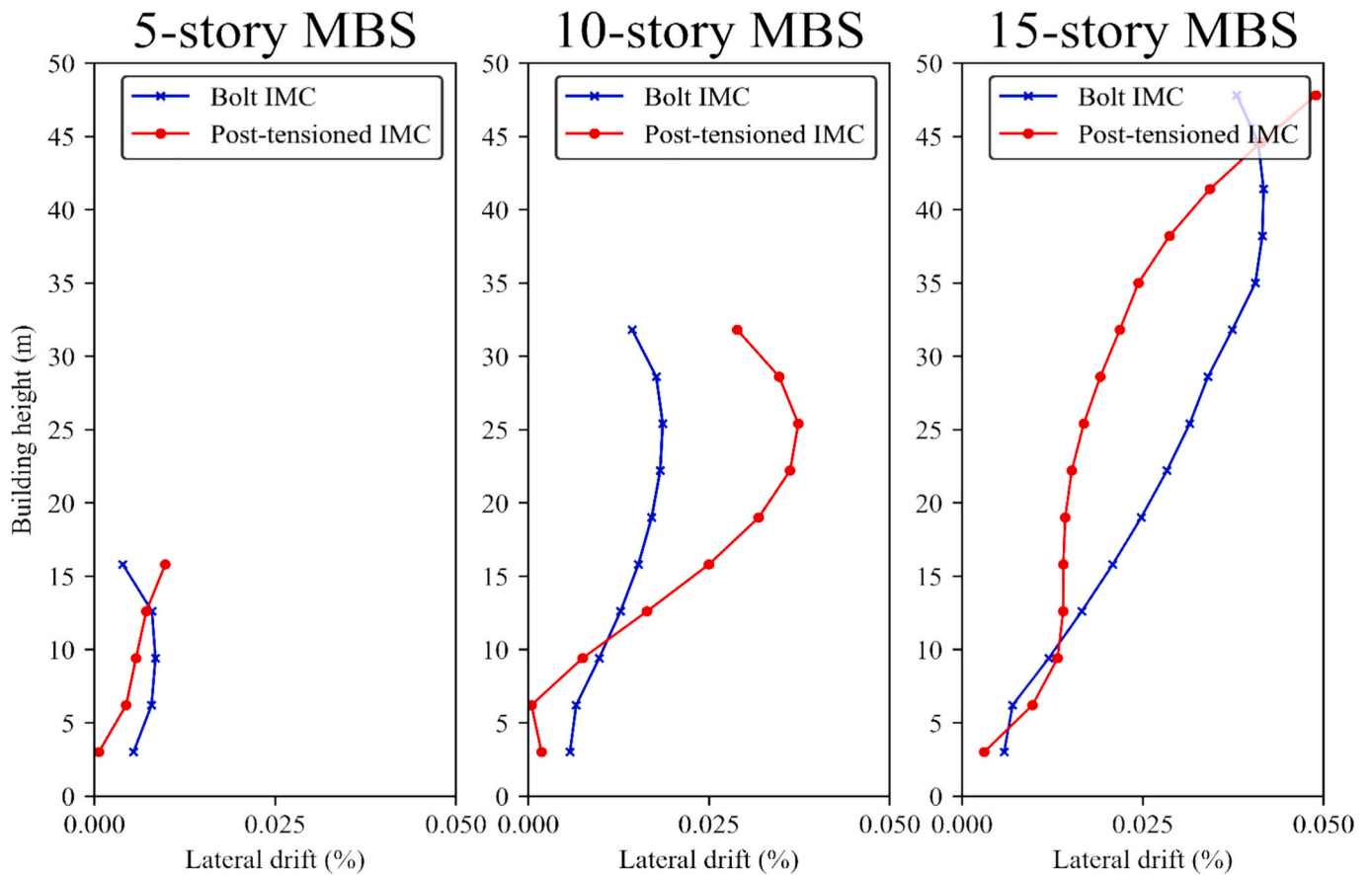
Fig. 9. Lateral inter-story drift ratios of the MBSs.
