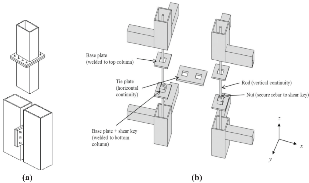
Fig. 4. Two types of IMCs used in this study: (a) Bolted IMCs [47], and (b) Post-tensioned rod [18].
