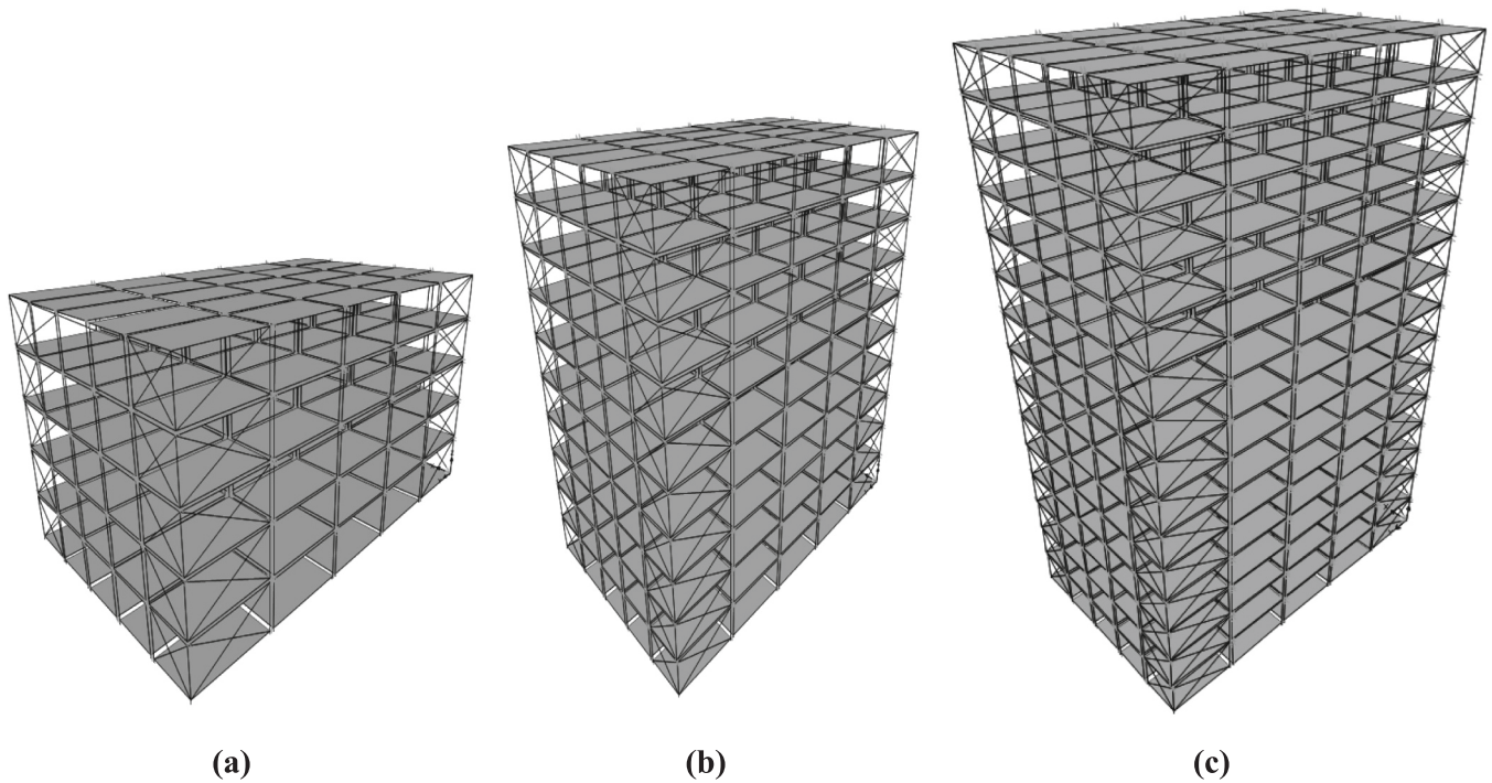
Fig. 6. 3D view of MBS case studies: (a) 5-story MBS, (b) 10-story MBS, (c) 15-story MBS.
