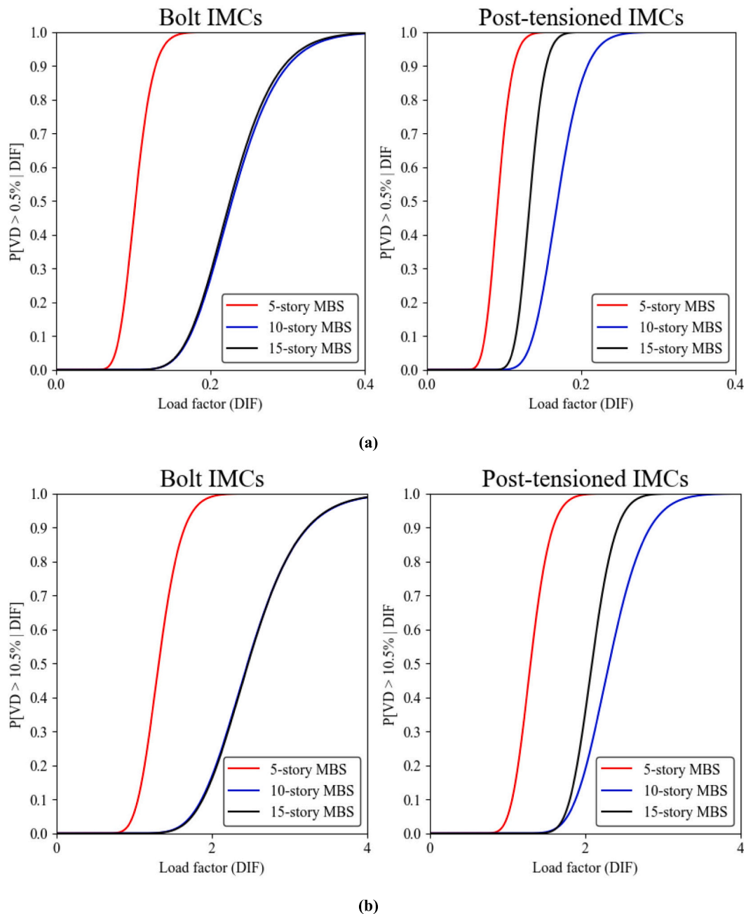
Fig. 15. Probabilistic demand models of MBSs for bolted and post-tensioned IMCs under progressive collapse scenario for (a) Significant limit state, and (b) Collapse limit state.
