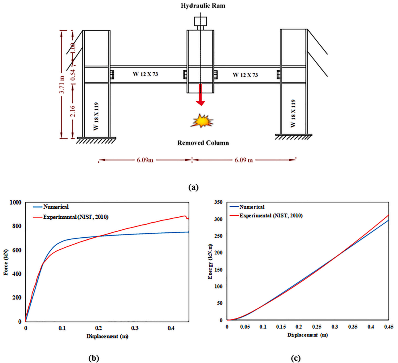
Fig. 7. Comparison of the experimental results and numerical results for progressive collapse scenario: (a) Details of test specimen, (b) Applied vertical load versus vertical displacements at center column, and (c) Cumulative energy versus vertical displacement at center column.
