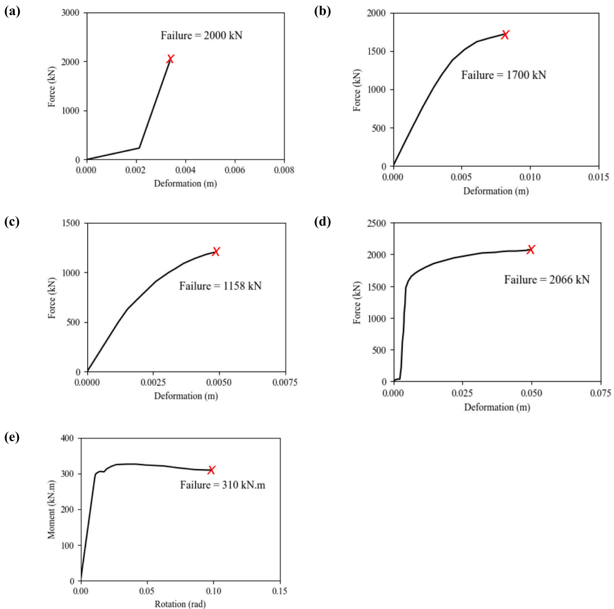
Fig. 5. The nonlinear behaviour of (a) Vertical connection in shear direction, (b) Vertical connection in axial direction, (c) Horizontal connection in axial direction, (d) Horizontal connection in shear direction, (e) Horizontal connection and Vertical connection in moment direction [47].
