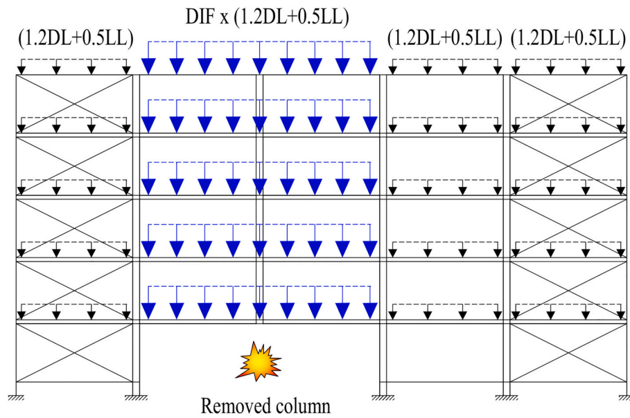
Fig. 8. Pushdown analysis of 5-story MBS model for progressive collapse scenario.
