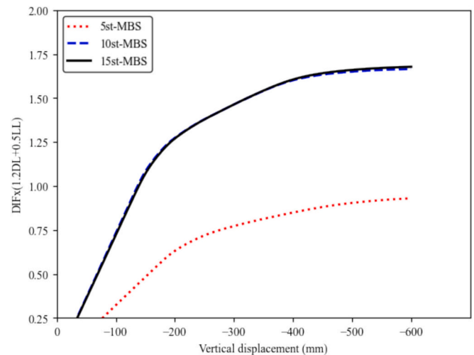
Fig. 12. Capacity curves of bolted IMCs for the MBSs.
