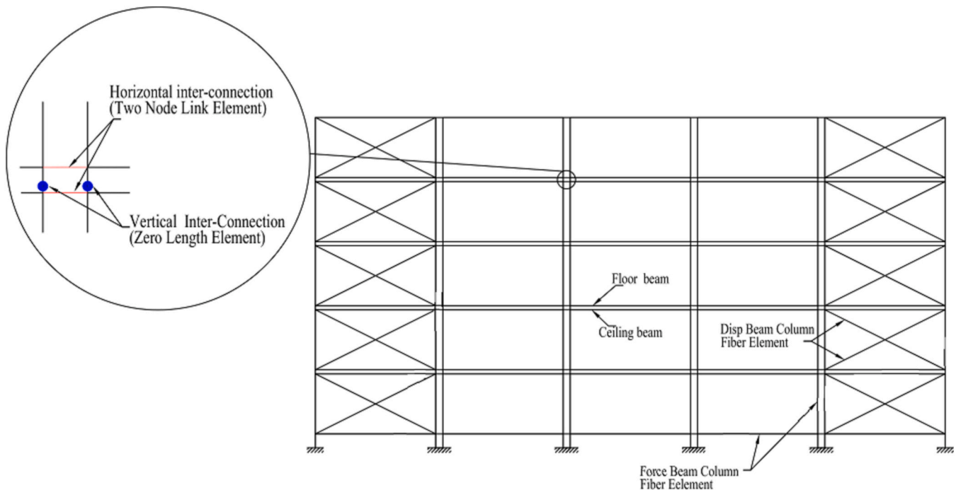
Fig. 3. Visual model of horizontal and vertical connections used in this study.
