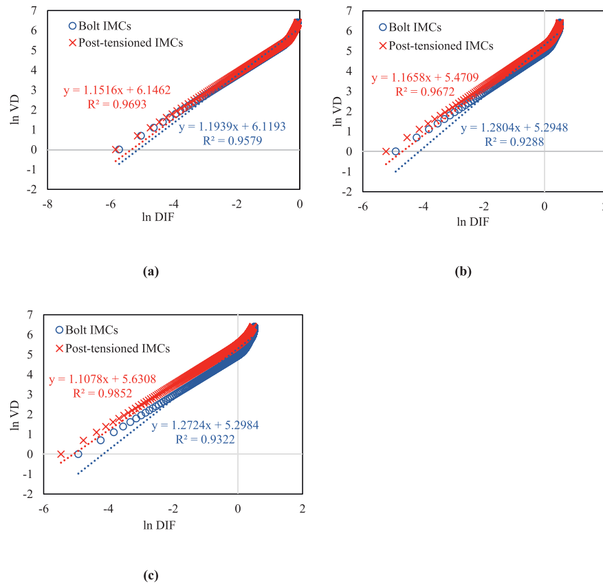
Fig. 14. Regression of the probabilistic demand model for (a) 5-story MBS, (b) 10-story MBS, and (c) 15-story MBS.
