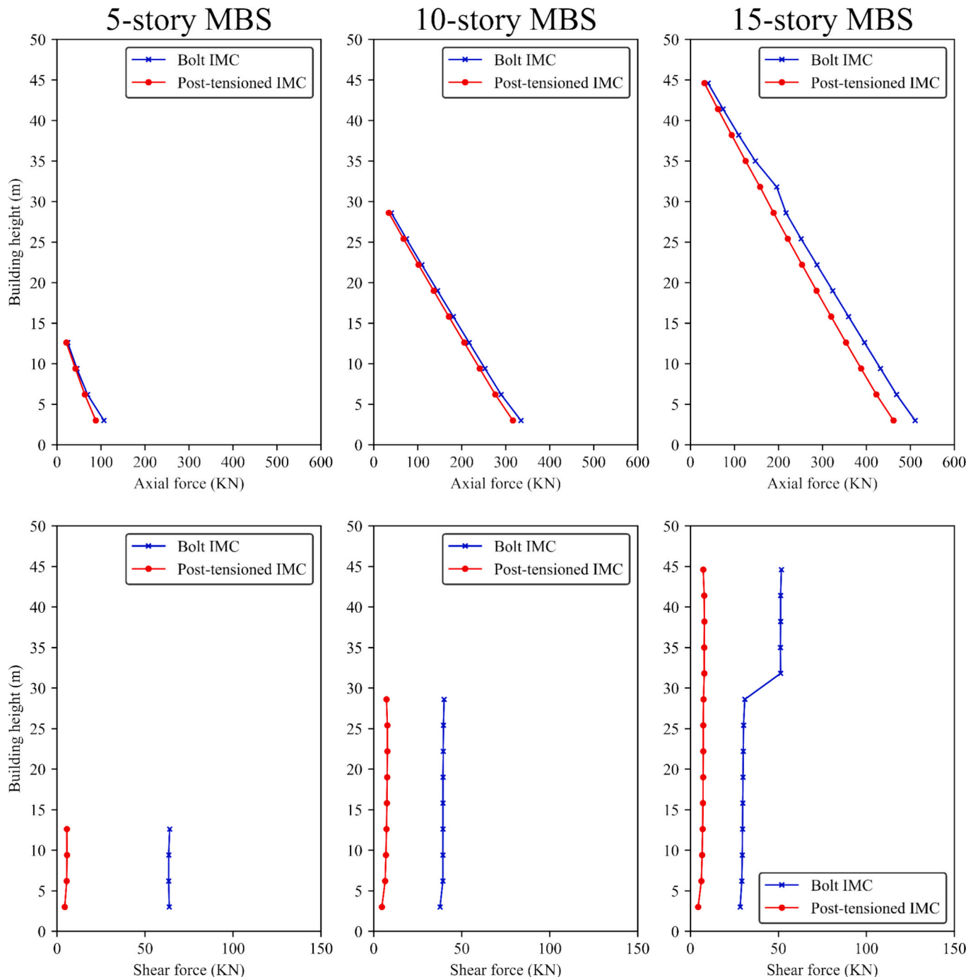
Fig. 10. Peak axial and shear forces in vertical IMCs for 5, 10, and 15-story MBSs.
