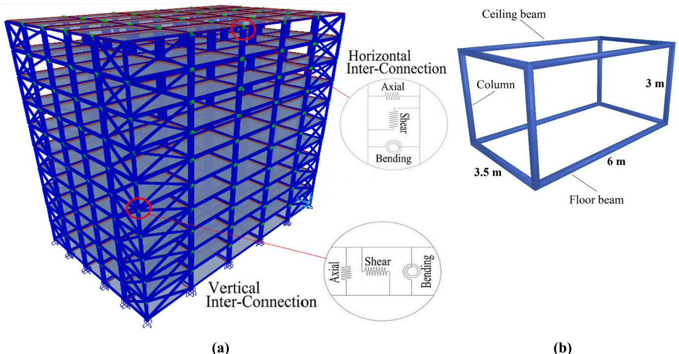
Fig. 2. 3D view of (a) 10-storey steel modular building system (MBS) and (b) Single module.
