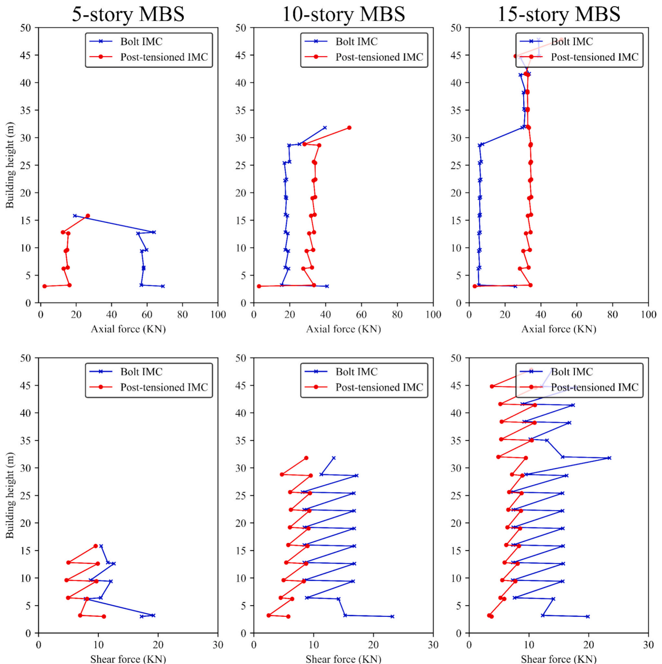
Fig. 11. Peak axial and shear forces in horizontal IMCs for 5, 10, and 15-story MBSs.
