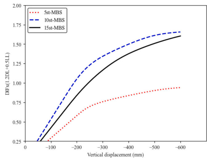
Fig. 13. Capacity curves of post-tensioned IMCs for the MBSs.
