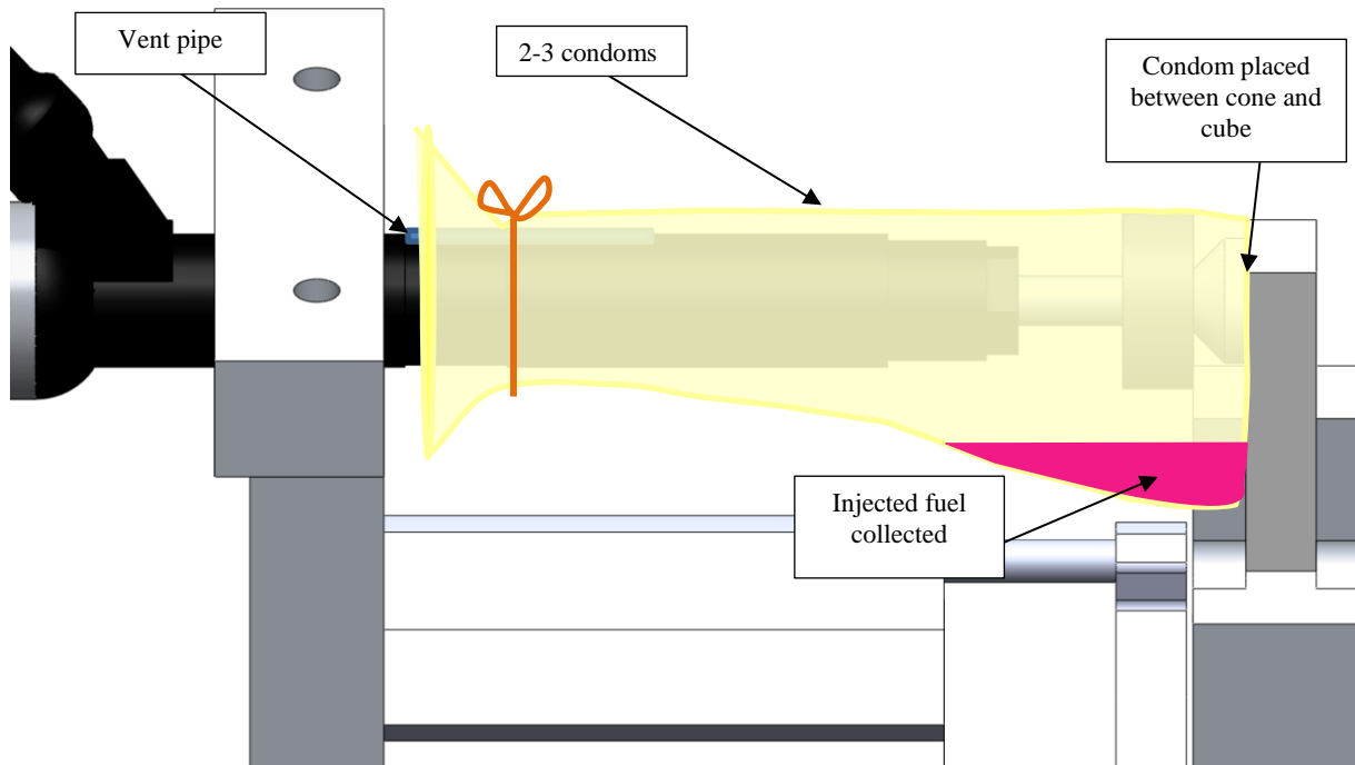
Figure 6.11 Modified nozzle injector- condom injected mass collection setup
