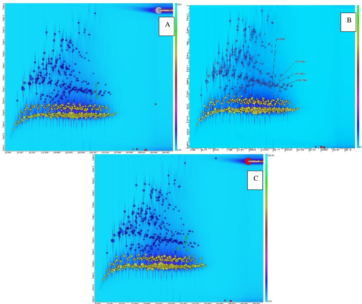
Figure 4.32 Figures obtained from the GC x GC analysis of Shell Flitwick A-initial sample, B- forty hours cavitating flow sample an C- forty hour discontinuous heat test sample.
