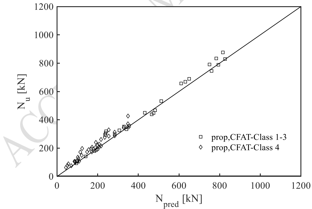
Figure 16: Comparison of experimental and numerical ultimate loads with proposed design strengths for CFAT columns.
