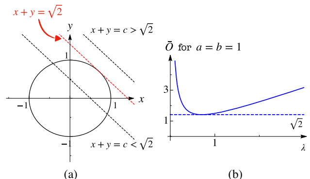
FIG. 1. (a) The geometric solution of problem \max\{x+y|x^2+y^2 \leq 1\} . (b) The dual function \bar{\mathcal{O}}(\lambda) = \lambda + 1/(2\lambda) of the same maximization problem. The minimum value is attained for \lambda = 1/\sqrt{2} and coincides with the optimal value of the maximization problem.
