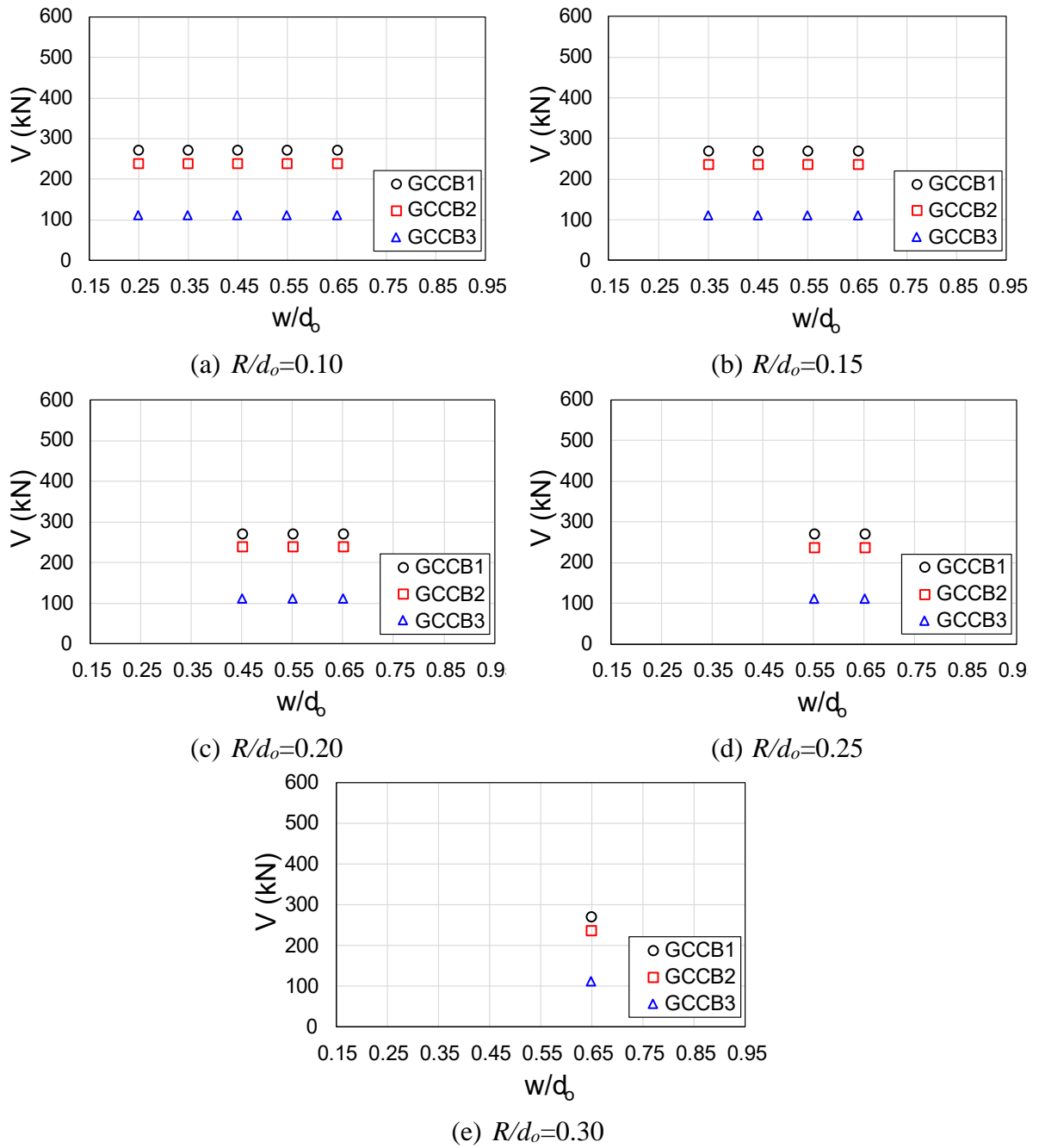
336 Fig. 26: Comparison of parameters w/d_o and R/d_o for GCCB1, GCCB2 and GCCB3 models 337 ( d_o/H=0.80 ).
