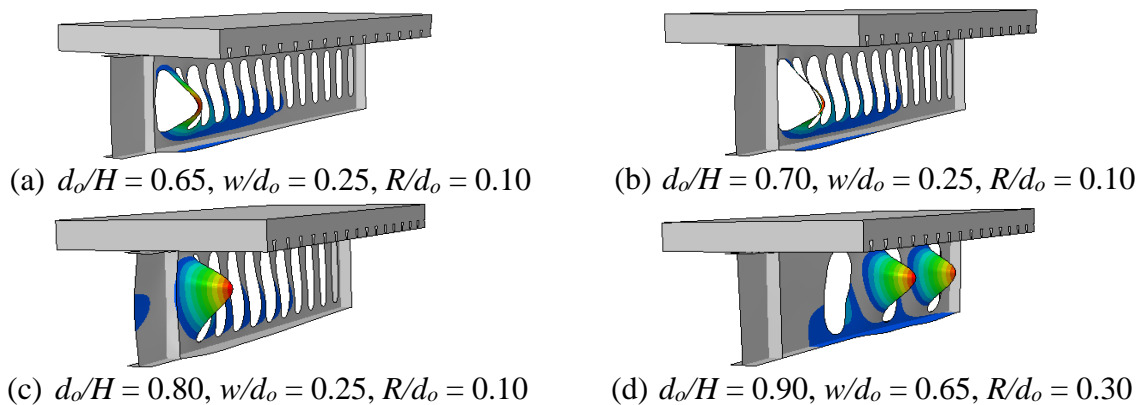
21 Fig. 10: Buckling modes of GCCB2 models
