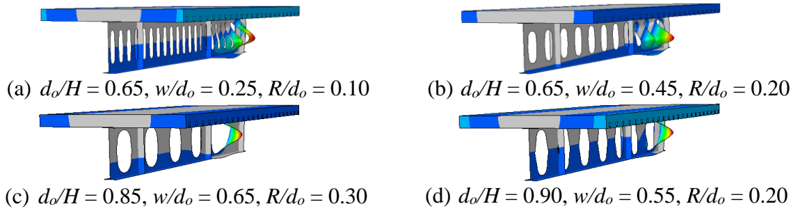
26 Fig. 11: Buckling modes of GCCB3 models
