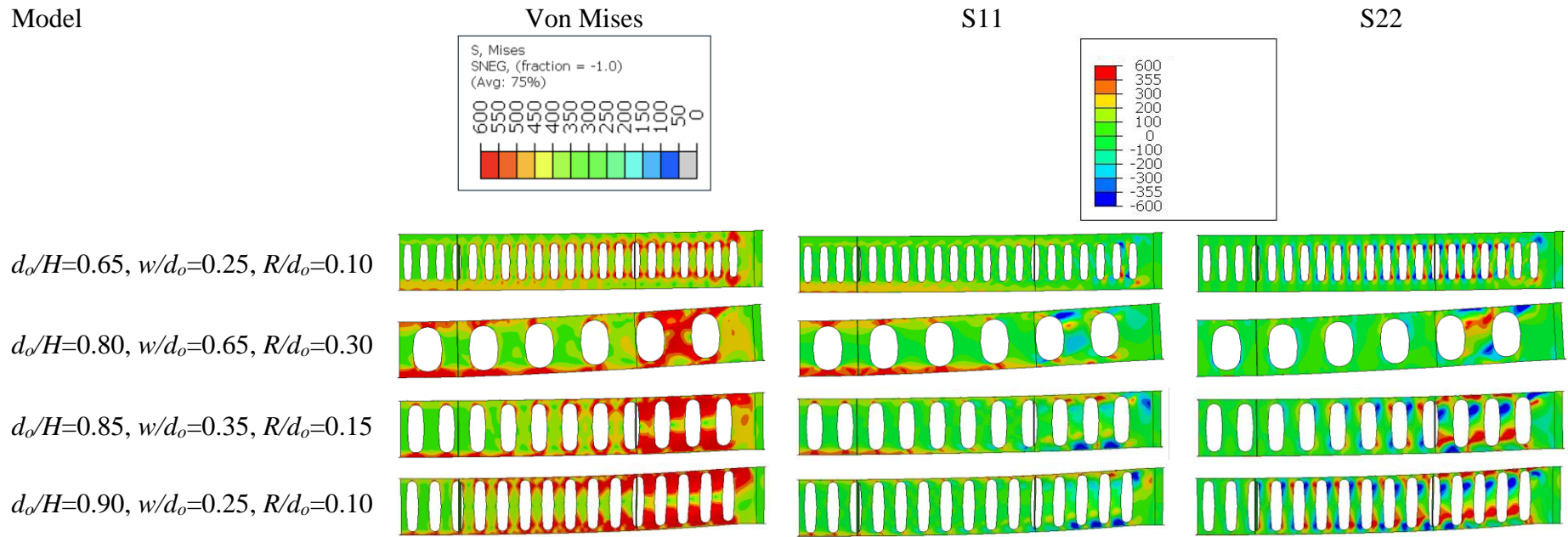
Fig. 21: Stresses in MPa, GCCB3.
