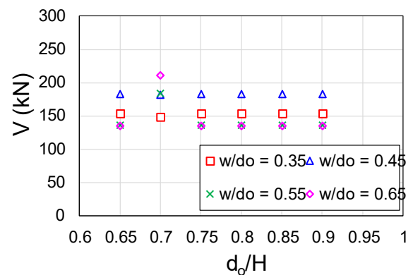
(b) R/d_o = 0.15
