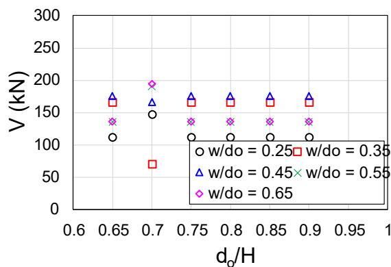
(a) R/d_o = 0.10
