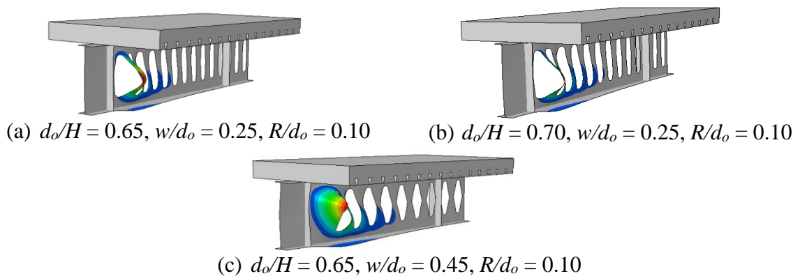
17 Fig. 9: Buckling modes of GCCB1 models
