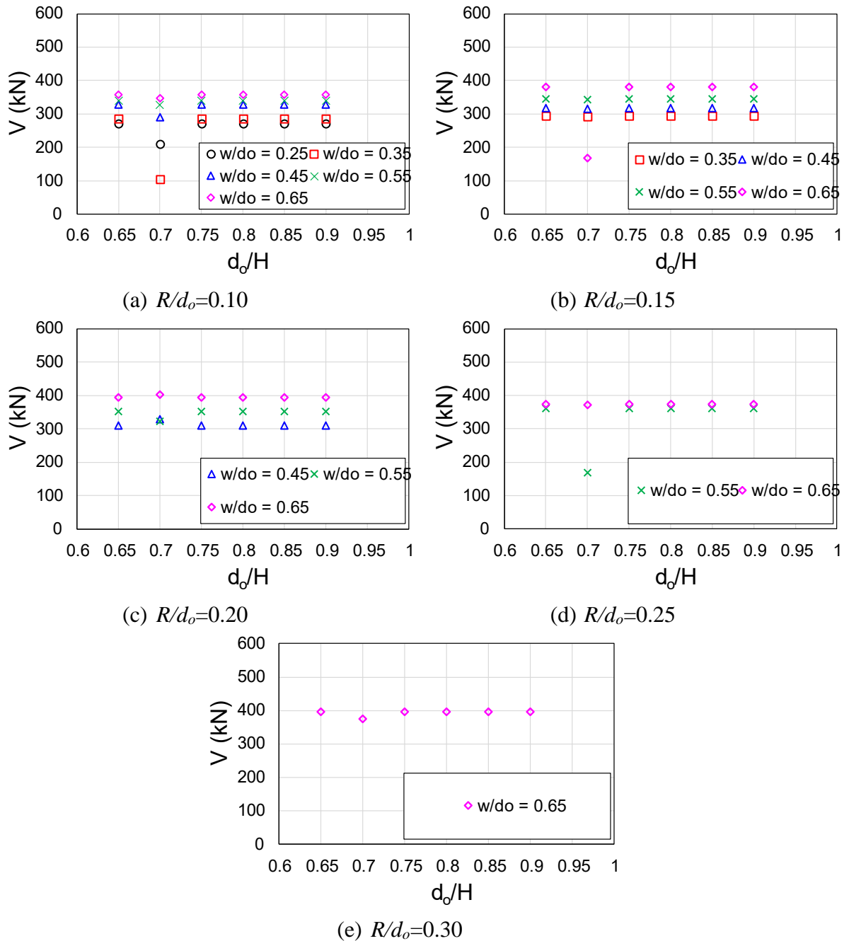
129 Fig. 16: Comparison of parameters for the GCCB1 models.
