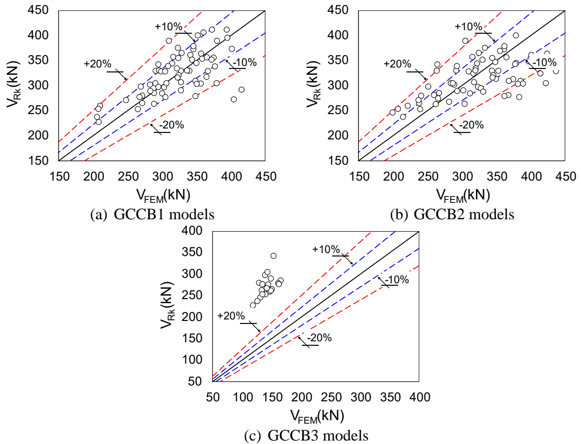
295 Fig. 24: Comparison between finite element models and predictions by Ferreira et al. [3], 296 considering buckling curve 'a'
