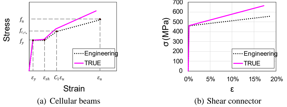
Fig. 2: Stress-strain relationship of steel models
