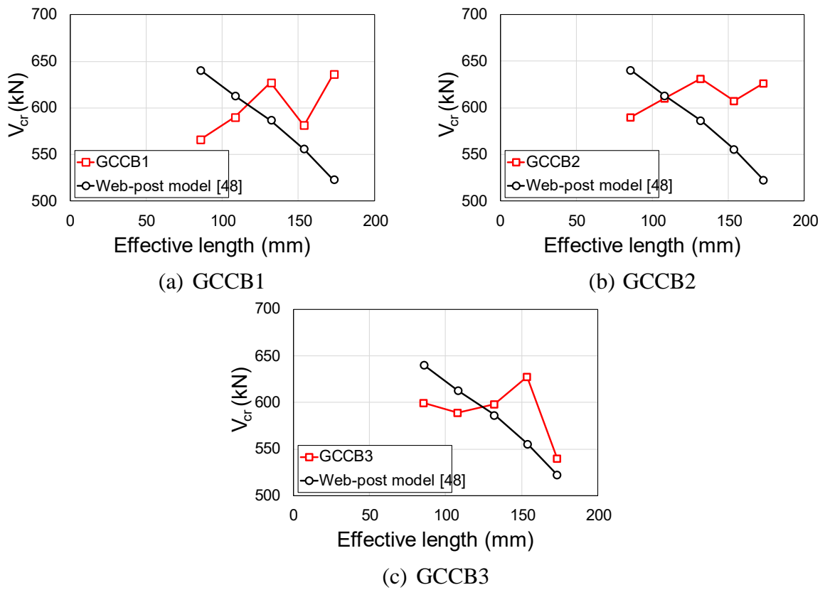
39 Fig. 12: Comparison between the effective length – web-post models [48] vs. composite beam 40 models.
