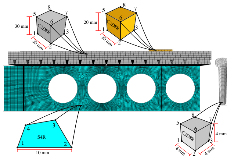
Fig. 4: FE discretisation of the concrete and shear connectors.
