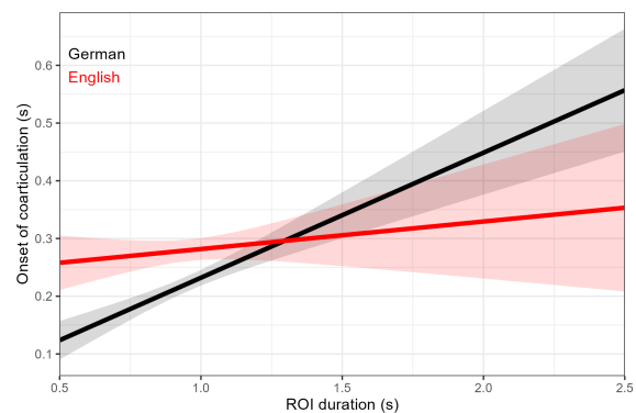
Figure 4: Model-predicted effect of ROI duration on onset of coarticulation (in s) in German (black) and English (red). Ribbons show \pm 2\text{SD} .
