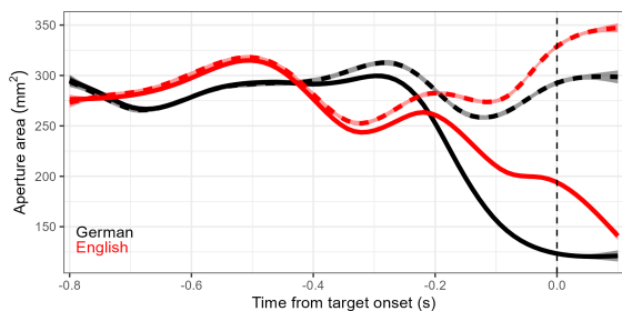
Figure 2: Overall aperture ( \text{mm}^2 ) from 800 ms before to 100 ms after target onset (rounded: solid, unrounded: dashed; German: black, English: red; ribbons show \pm 2\text{SD} ).
