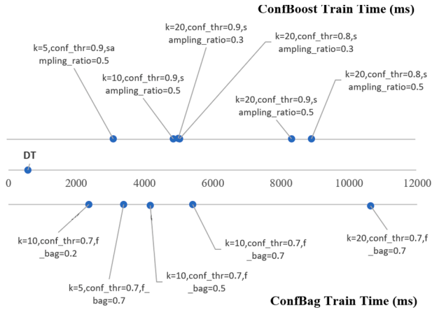
Fig. 5. Variation of Train Time for different instances of ConfBag (down in the figure) and ConfBoost (up) built over Decision Trees as base estimator (DT, middle of the plot).
