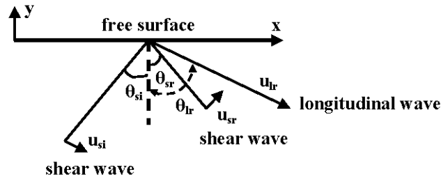
Figure 2.6. Shear wave incident on a free surface.
