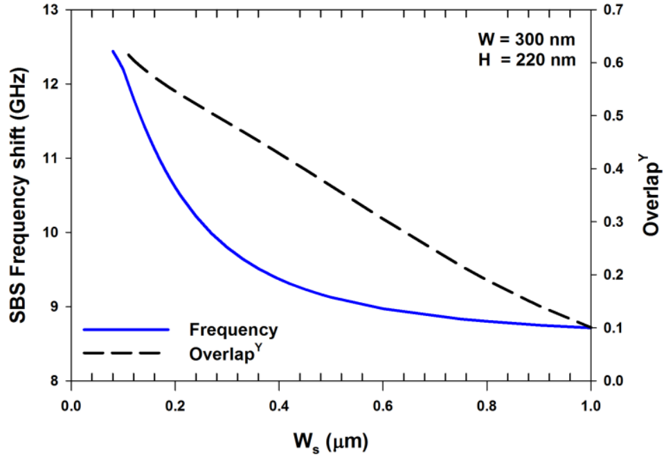
Figure 6.12. Variation of W_s with overlap integral and SBS frequency shift (GHz).
