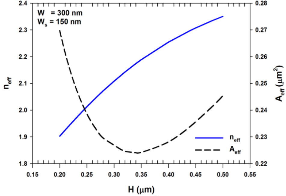
Figure 6.14. Variation of H with n_{\text{eff}} and A_{\text{eff}} ( \mu\text{m}^2 ).
