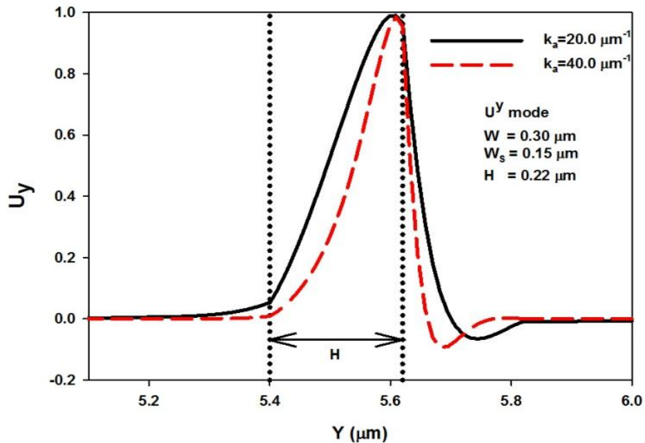
Figure 6.6. Variation of displacement vector U_y of the U^y mode along the y -axis at k=20.0 \mu\text{m}^{-1} and k=40.0 \mu\text{m}^{-1} .
