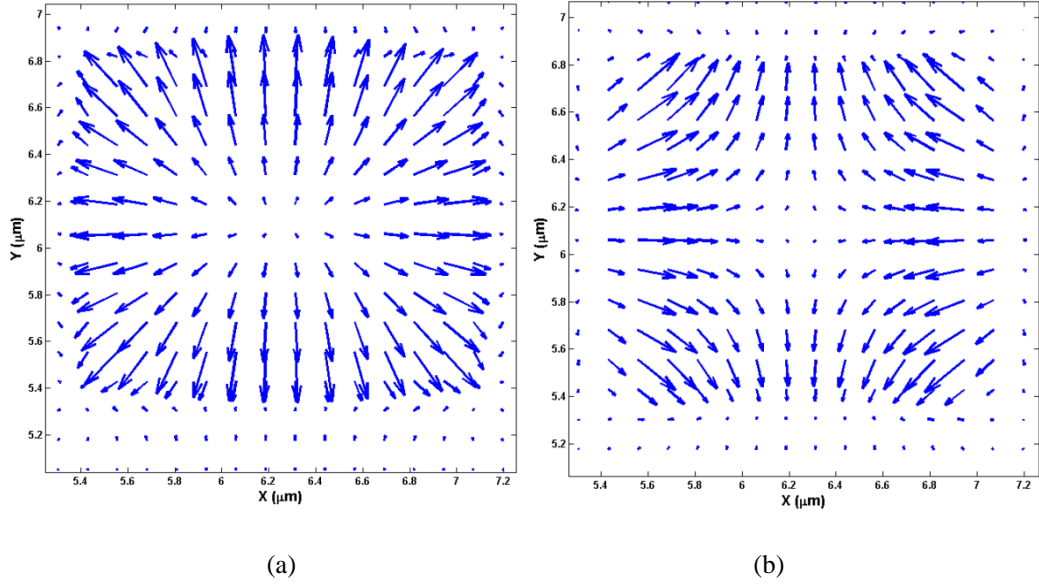
Figure 5.32. Vector plot U_t of (a) Radial mode (R1) (b) Torsional-Radial mode (TR1) at k = 10.0 \mu\text{m}^{-1} .
