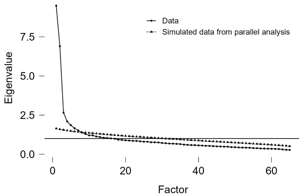
Fig. 1 Results from Parelle analysis shows seven factor structure.
