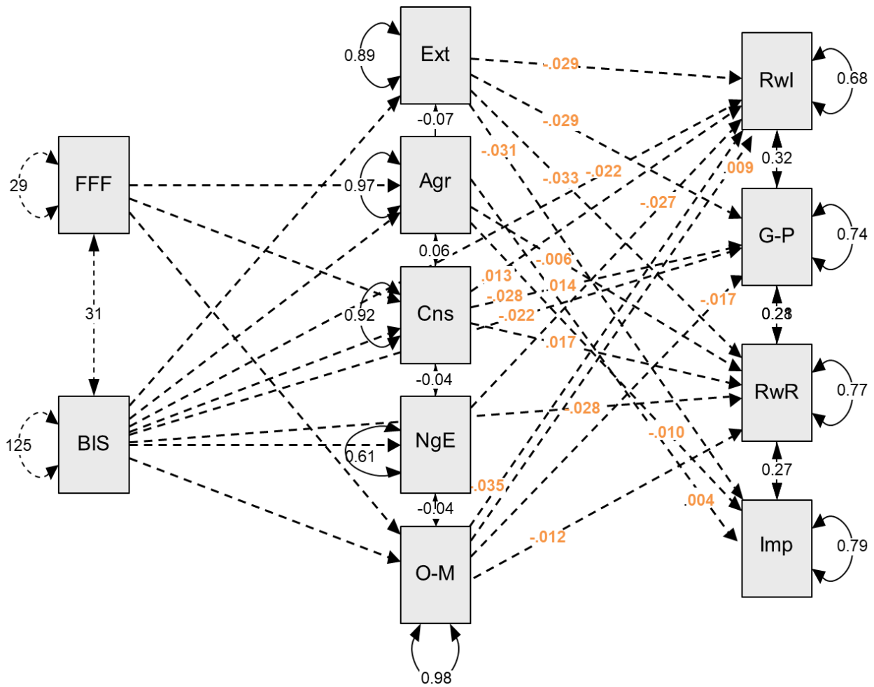
Fig.2 shows that personality traits mediated associations between FFFS and BIS, with BAS subscales
