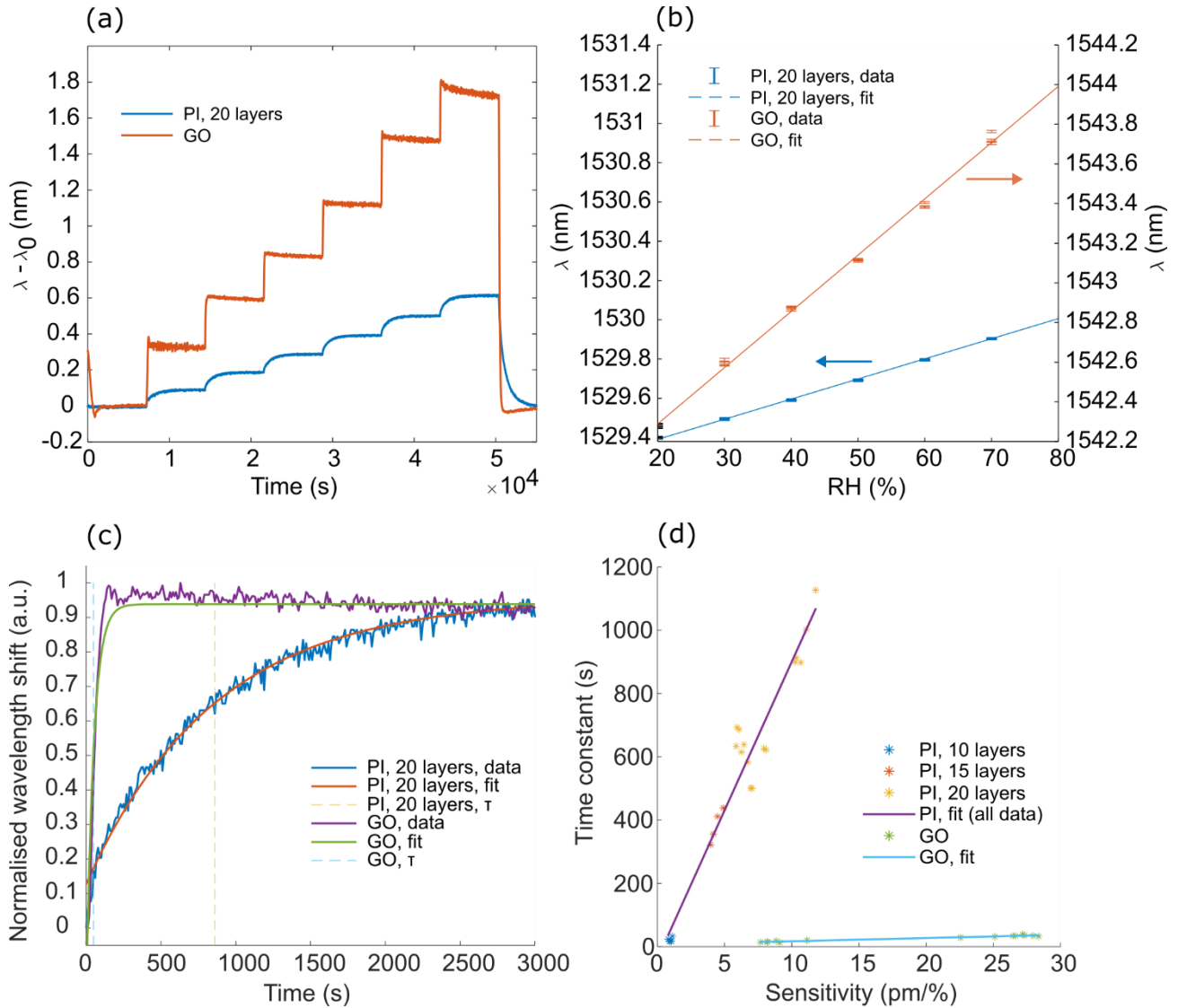
Figure 1: (a) Wavelength shift (initial wavelength \lambda_0 subtracted) versus time for representative polyimide (PI) and graphene oxide (GO) coated relative humidity (RH) sensors during calibration with RH steps from 20% to 80%; (b) Calibration curves obtained from the data shown in (a) for PI and GO sensors; (c) Wavelength data, baseline-subtracted and normalized, versus time during a step change from 40% RH to 50% RH, with fitted lines used for estimating the time constant \tau ; (d) Time constant versus RH sensitivity coefficient for PI and GO coated sensors, showing data for all sensors tested.
