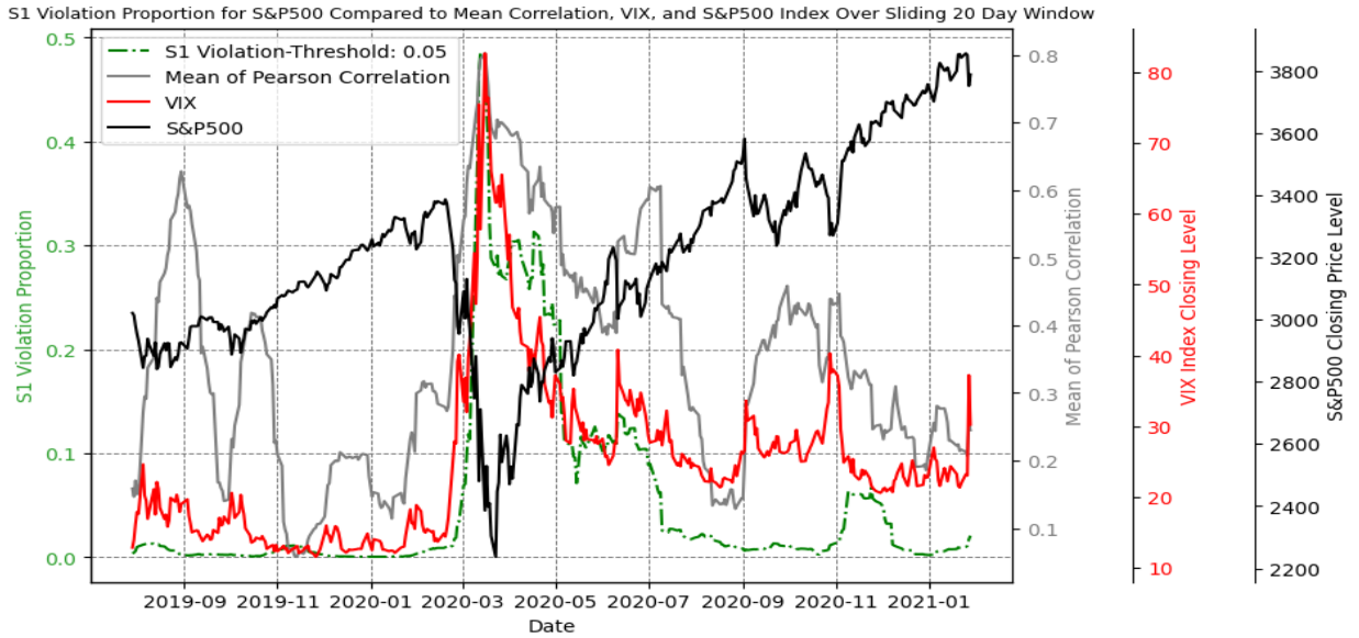
Figure 5: Average of pairwise Pearson correlations of price returns vs VIX, S_1 -violation proportion and daily closing price level of S&P 500 index: COVID-19 Crisis (U.S.)
