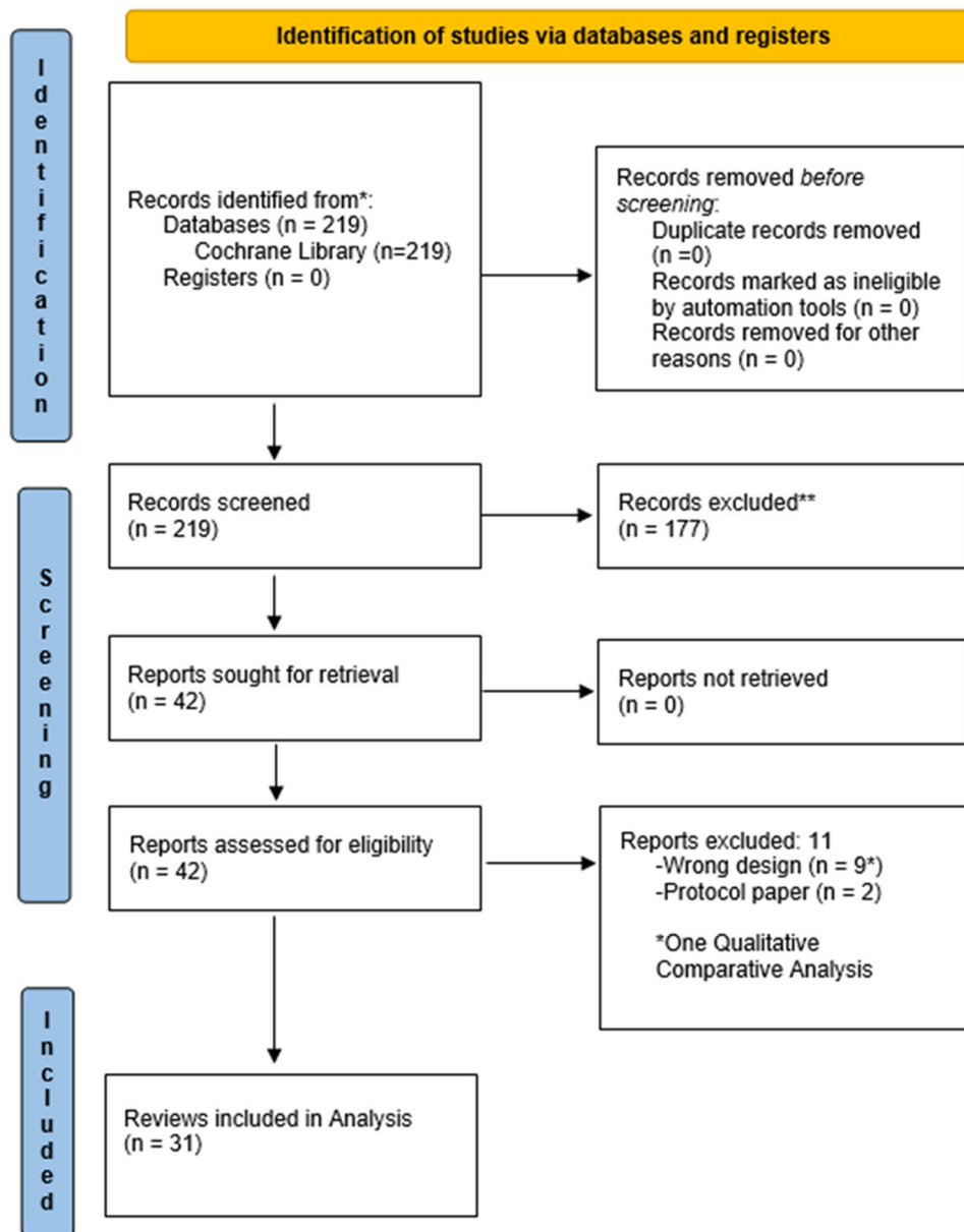
FIGURE 3 PRISMA flow-chart.
