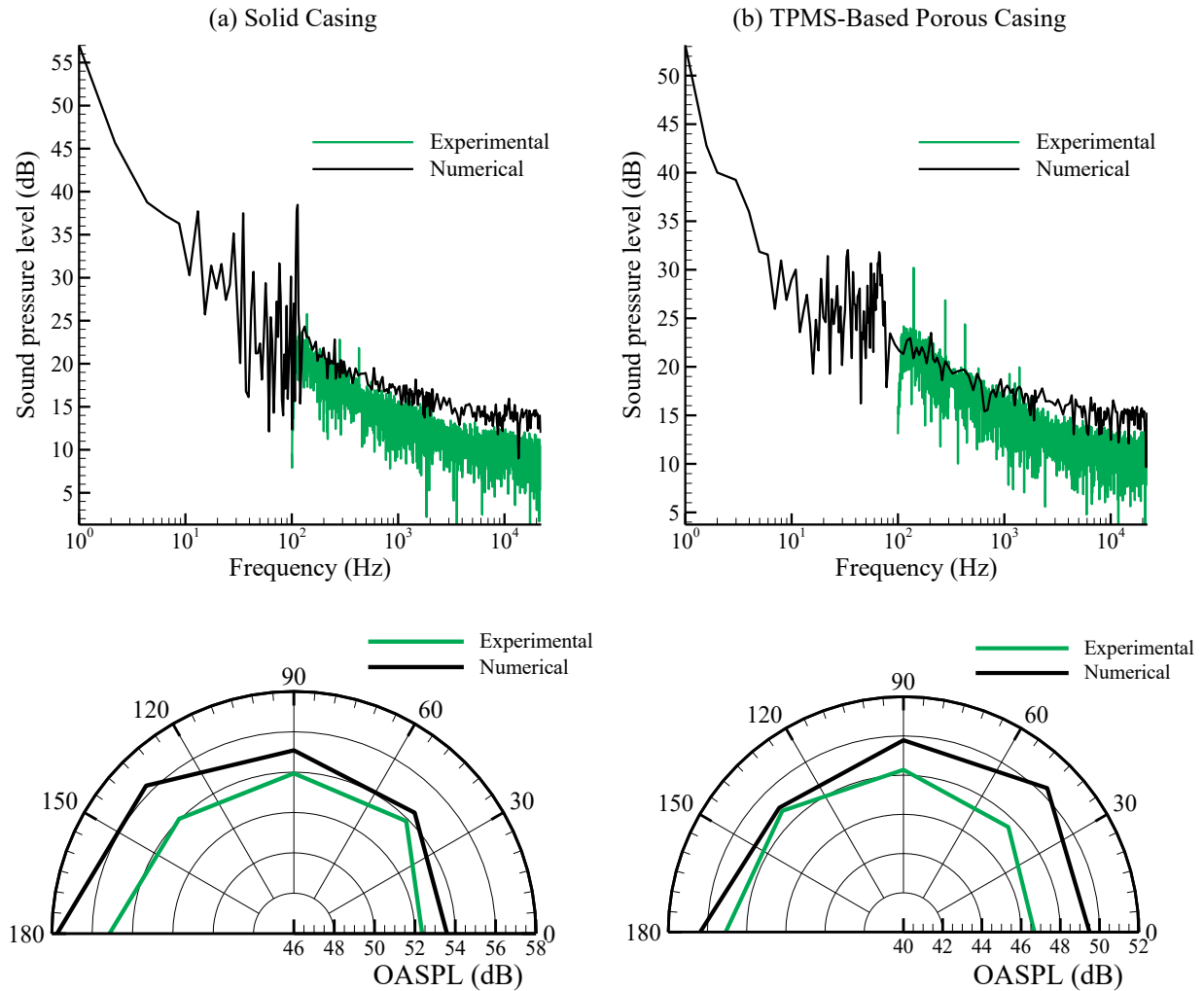
Figure 6. Numerical simulation validation: measurements were taken at 0.8 m distance and a 45° angle to the horizontal axis, at a rotational speed of 1200 rpm.
