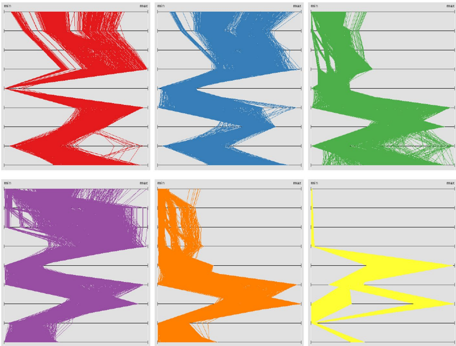
Fig. 16 Screenshots of the PCP display show the distributions of the feature values separately for each class: 1) red - straight movement; 2) blue - curved movement; 3) green - trawling; 4) purple - port-connected; 5) orange - near port; 6) yellow - anchored
