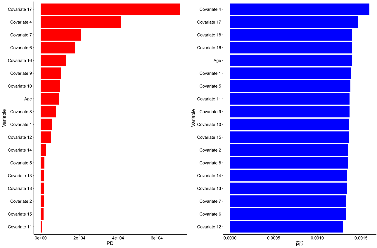
Fig. 5. First-order ( PD_i ) and total sensitivity ( \bar{PD}_i ) of unawareness prices, for each covariate in the real world dataset.
