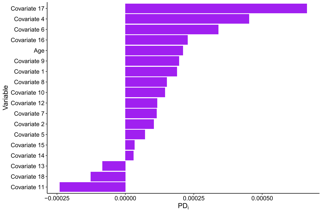
Fig. 6. CEN-SHAP attributions of proxy discrimination, implementing Shapley values (12).
