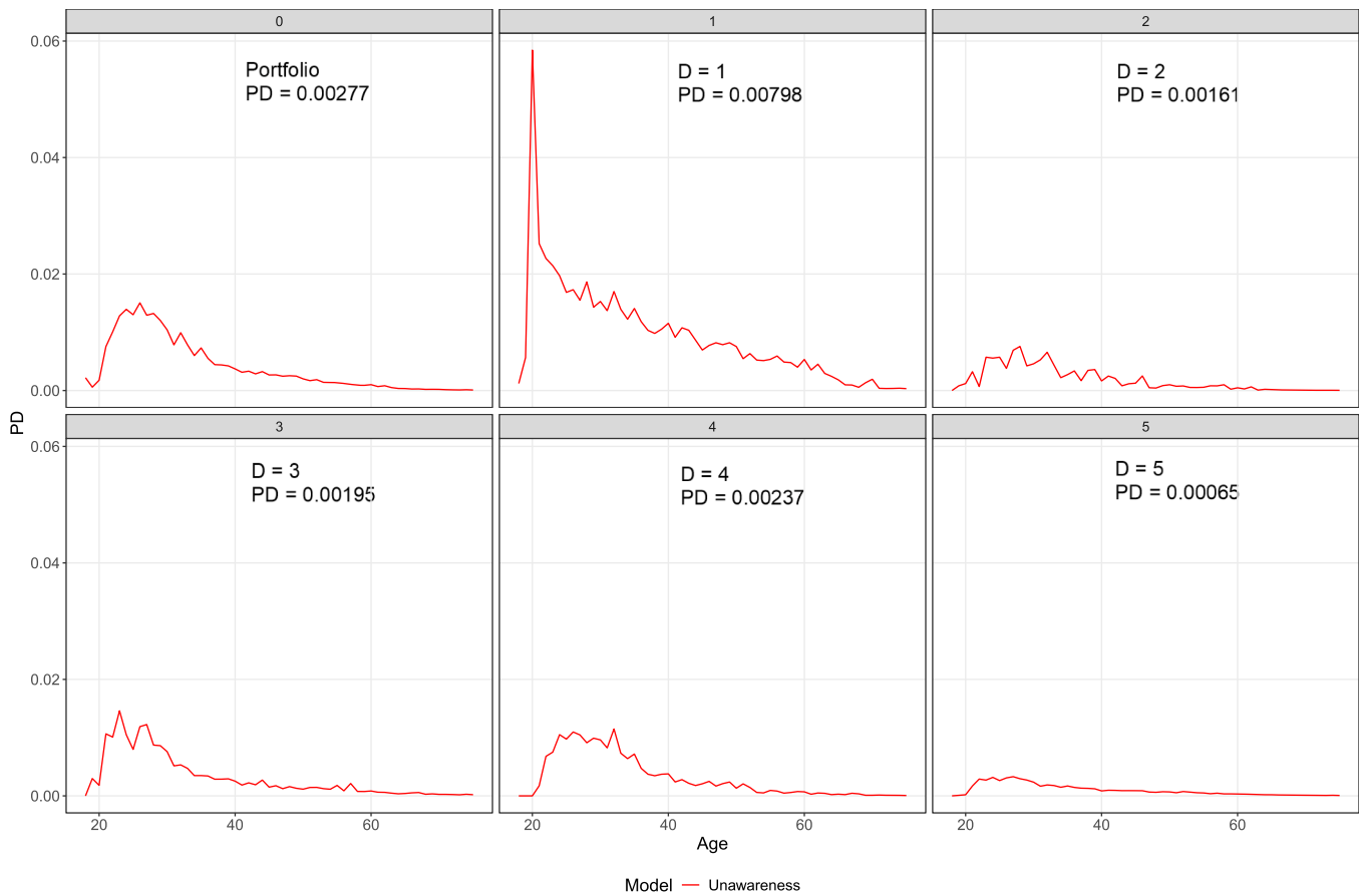
Fig. 4. Proxy discrimination metric PD_{|Age, D}(a, d) evaluated for the age variable, for each ethnicity code separately and for the portfolio as a whole (Eq. (18)).
