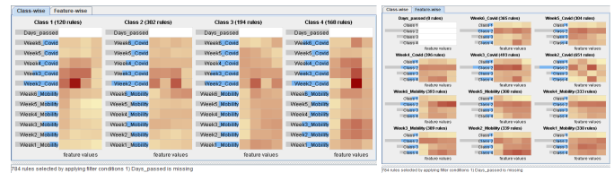
Fig. 12: Feature distributions over rules that do not involve Days_passed.
