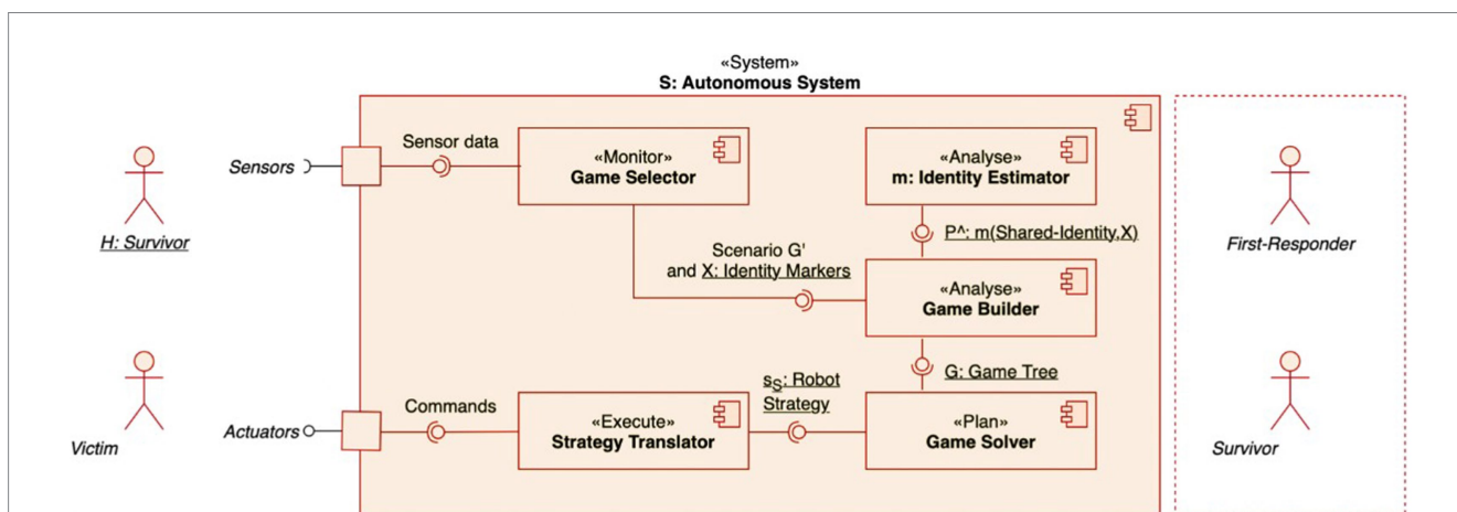
FIGURE 1 MAPE-K framework for the identity-adaptive autonomous agent. Component diagram of our adaptive architecture: the game selector triggers an identity-driven scenario G that there is an injured individual close to another survivor and sends identity marker information X (linguistic data) to the game builder. This component assembles the game tree G incorporating the identity probabilities P produced by the identity estimator. The game solver calculates the robot strategy sG that the strategy translator transforms into actionable commands.
