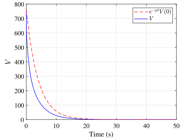
Fig. 7. Lyapunov function V generated by the proposed distributed observer in Scenario 1.
