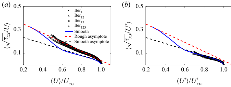
Figure 17. Effect of the different multiscale rough surfaces on (a) the total normalised streamwise rms profiles in the diagnostic-plot form as proposed by Alfredsson et al. (2011). (b) The same data with the modified scaling U' = U + \Delta U^+ and U'_\infty = U_\infty + \Delta U^+ proposed by Castro et al. (2013).
