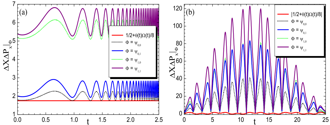
Figure 4: Uncertainties \Delta X \Delta P_x |_{\psi_{n,m-n}} versus the generalized lower bound (a) for background fields \theta(t) = \alpha e^{-\gamma t} and \Omega(t) = \beta e^{\gamma t} and (b) for background fields \theta(t) = \alpha \sin(\gamma t) and \Omega(t) = \beta \sin(\gamma t/2) . In both panels the constants are \alpha = 5 , \beta = 2 , \gamma = 2 , m = \hbar = \tau = \omega = 1 , \kappa = 1/4 and \mu = \sqrt{5/3} .
