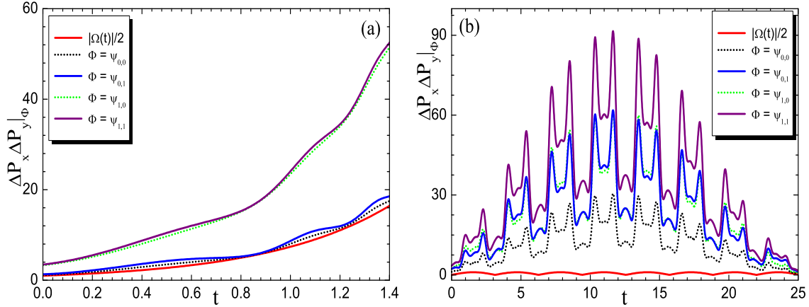
Figure 3: Uncertainties \Delta P_x \Delta P_y |_{\psi_{n,m-n}} versus the generalized lower bound (a) for background fields \theta(t) = \alpha e^{-\gamma t} and \Omega(t) = \beta e^{\gamma t} and (b) for background fields \theta(t) = \alpha \sin(\gamma t) and \Omega(t) = \beta \sin(\gamma t/2) . In both panels the constants are \alpha = 5 , \beta = 2 , \gamma = 2 , m = \hbar = \tau = \omega = 1 , \kappa = 1/4 and \mu = \sqrt{5/3} .
