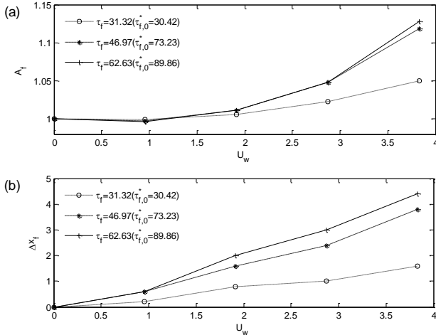
Fig. 10 Amplification factor A_f (a) and shift distance \Delta x_f (b) as a function of wind speeds in the cases with different \tau_{f,0}^* ( \omega_{\min} = 0.5 , \omega_{\max} = 1.4 , N=32 , a_n = 0.008 , x_f = 15 )
