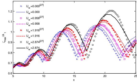
Fig. 3 Comparison of maximum elevation recorded at different positions ( \omega_{\min} = 0.8 , \omega_{\max} = 1.6 , N=32 , a_n = 0.00575 , x_f = 15 , \tau_f = 46.97 ; the superscript in the legend represents the results from QALE-FEM/StarCD approach in reference [27])
