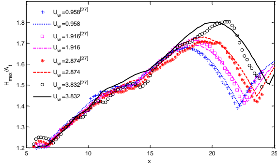
Fig. 2 Comparison of maximum wave height recorded at different positions ( \omega_{\min} = 0.5 , \omega_{\max} = 1.4 , N=32 , a_n = 0.008 , x_f = 12.5 , \tau_f = 46.97 ; the superscript in the legend represents the results from QALE-FEM/StarCD approach in reference [27])
