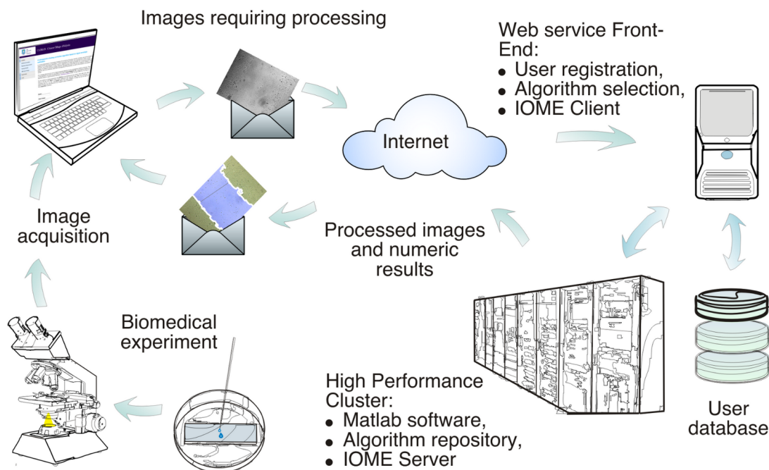
Fig. 1 Graphical description of CAIMAN
