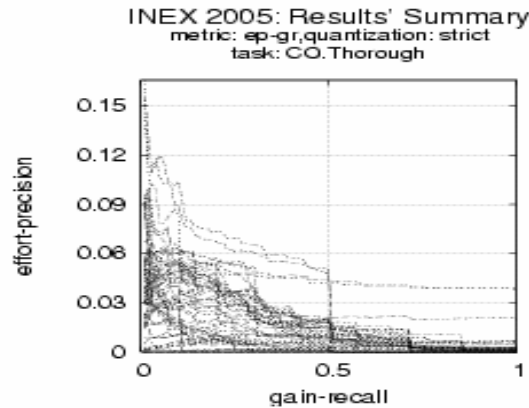
Fig. 3 Metric ep-gr, Quantization: strict,Overlap=off
