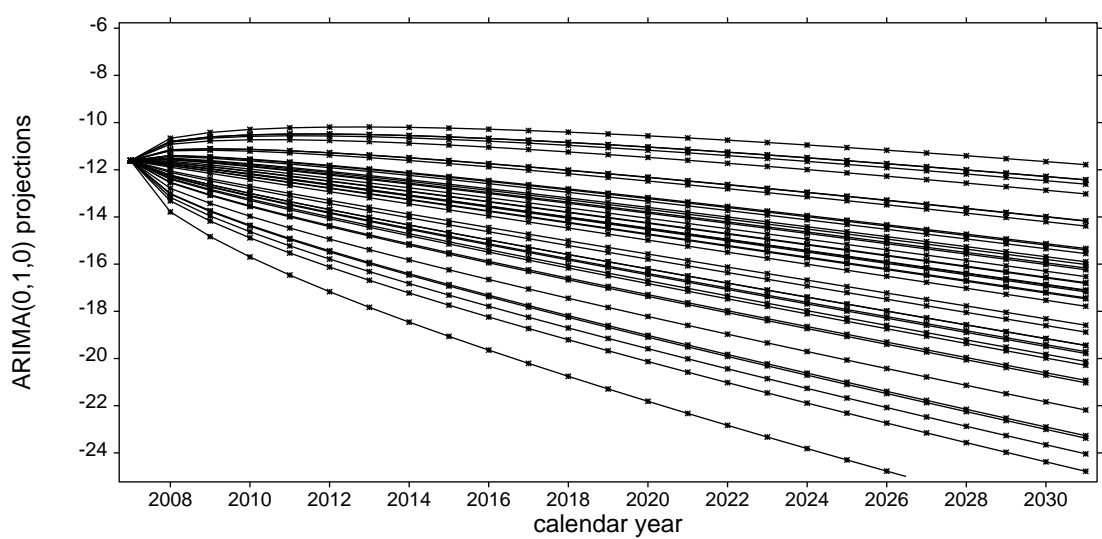
Algorithm 1: 40 simulations
