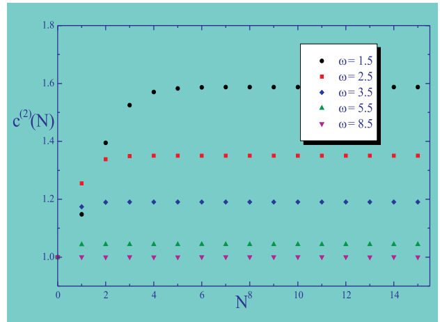
Figure 5: Ultraviolet Virasoro central charge c^{(2)} as a function of N .
