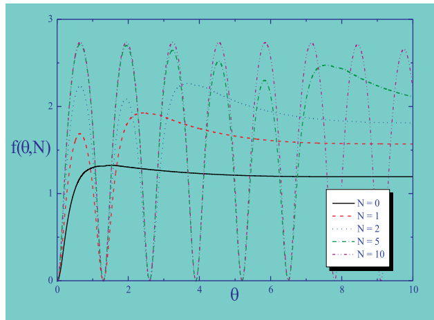
Figure 2: Absolute value squared of the two particle form factors f(\theta, N) = |\hat{F}_2^{\Theta}(\theta, N)|^2 / (2\pi)^2 as functions of the rapidity for different values of N for \omega = 1.3 and x = 0.1 .
