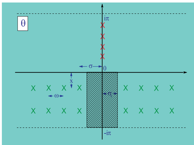
Figure 1: The poles of the blocks \{x\}_{\theta, \ell}^{\sigma} are the crosses in the sheet -\pi \leq \text{Im } \theta \leq 0 . The crosses on the positive part of the imaginary axis are associated, as usual, with stable particles. For equal masses of the stable particles the threshold (16) is \sigma_t = \text{arccosh}[(3 - \cos \pi x)/(1 + \cos \pi x)] .
