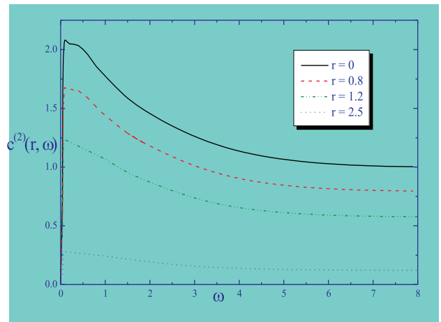
Figure 6: Ultraviolet Virasoro central charge c^{(2)} as a function of \omega .
