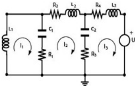
Figure 1: Initial RLC network
