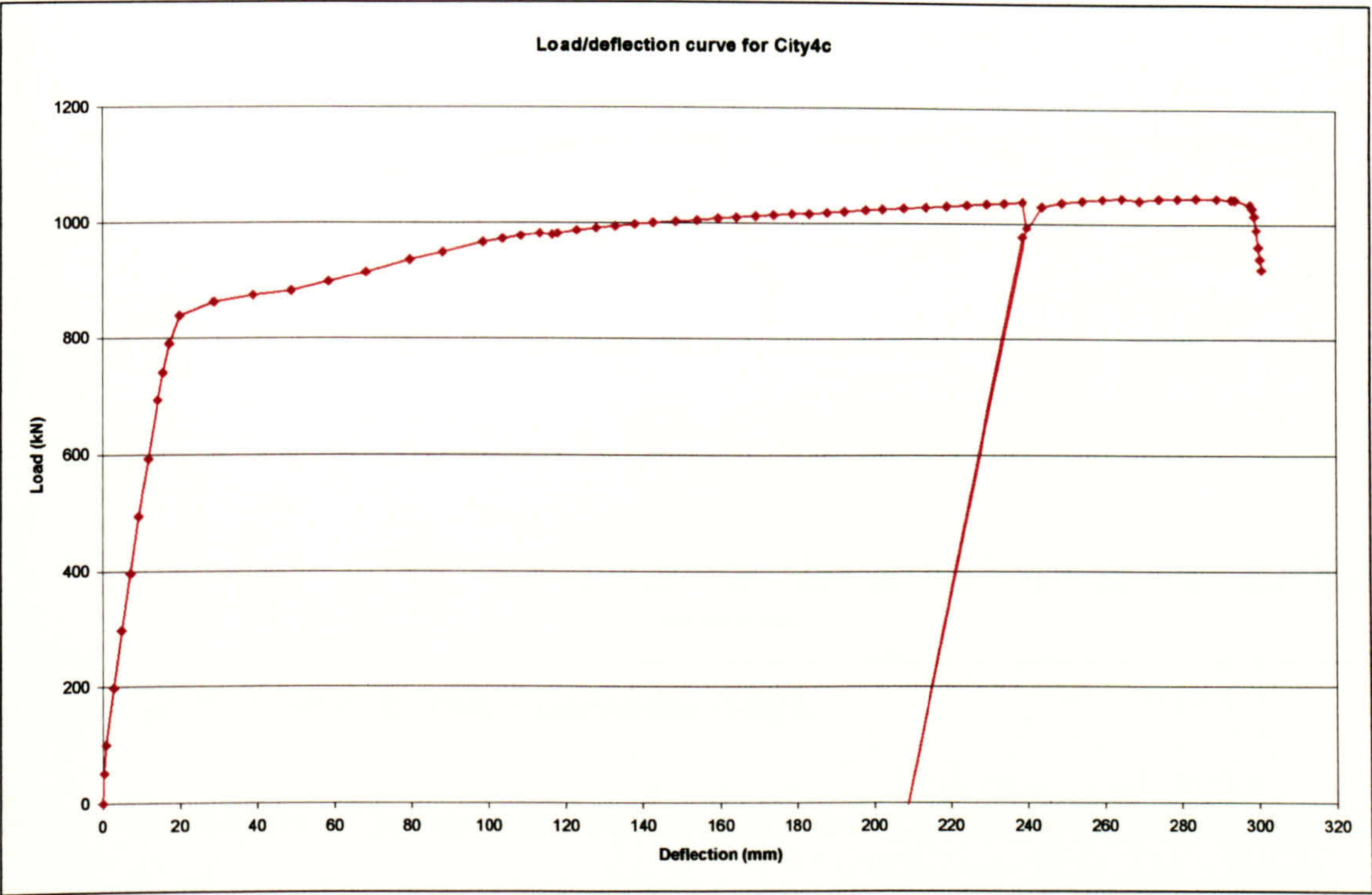
Figure 3.14 Load deflection curve for City4c.
