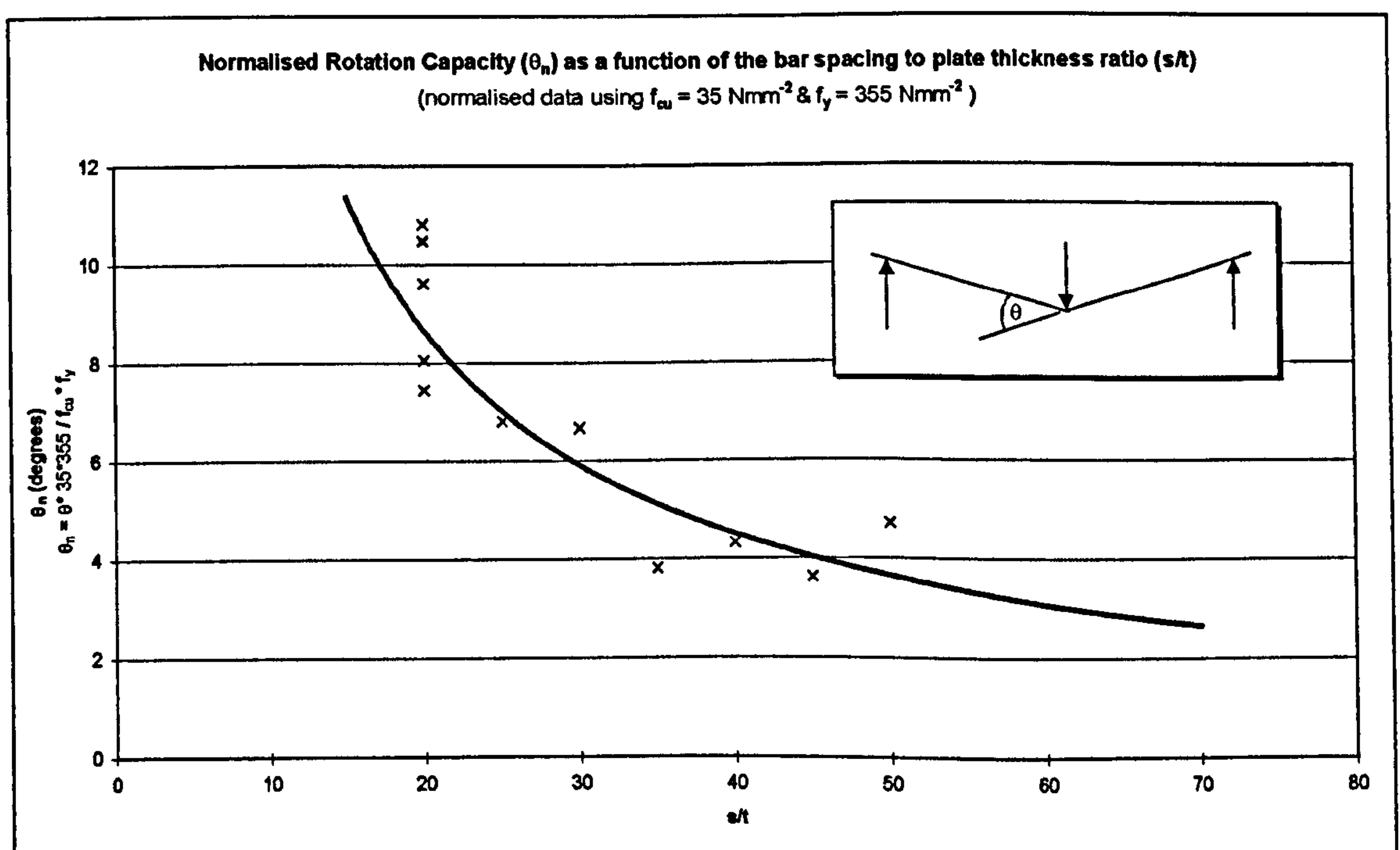
Figure 3.16. Rotation of Bi-Steel panels at buckling.
