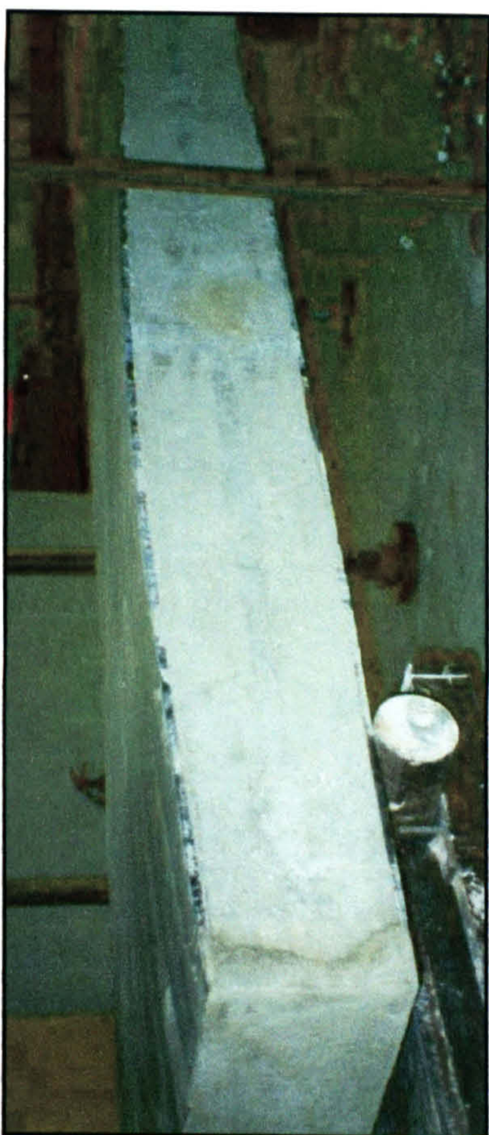
Plate B2c. Bulge in Stud2 caused by inadequate formwork.
