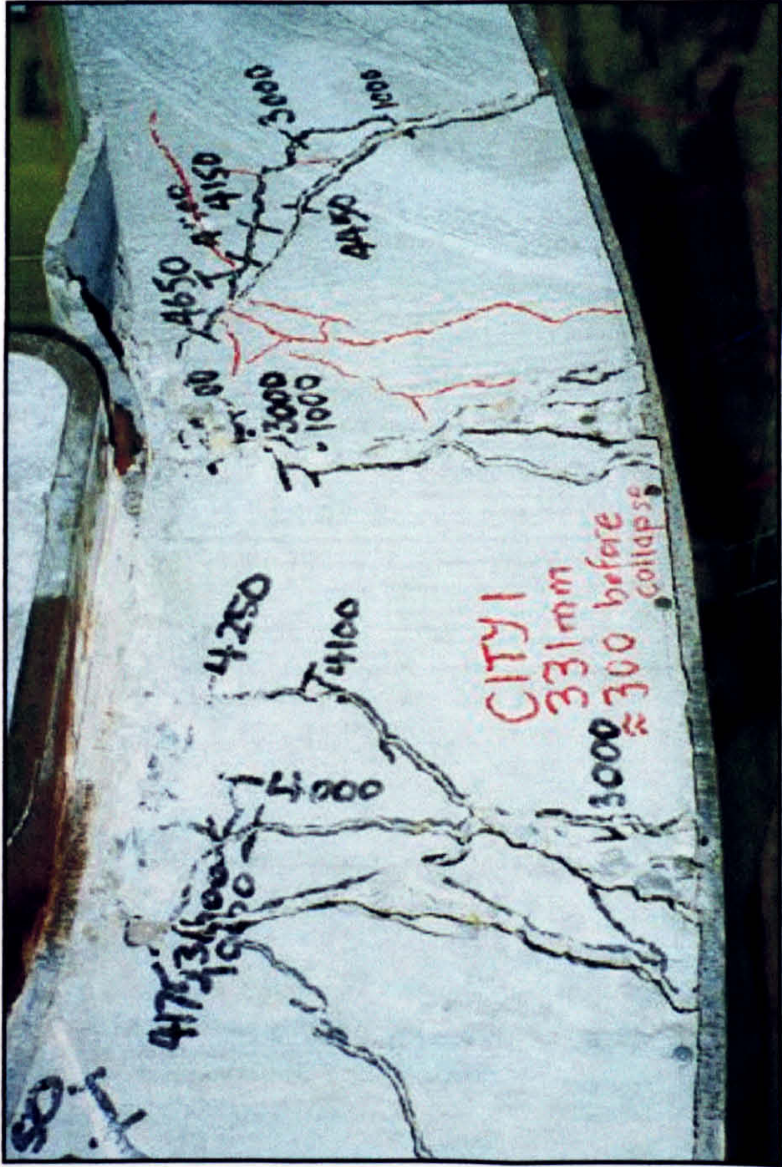
Plate B1a. Close-up of failed area showing concrete cracks originating from connector locations. Crack progression is marked in black for load (psi) and red for deflection (mm).
