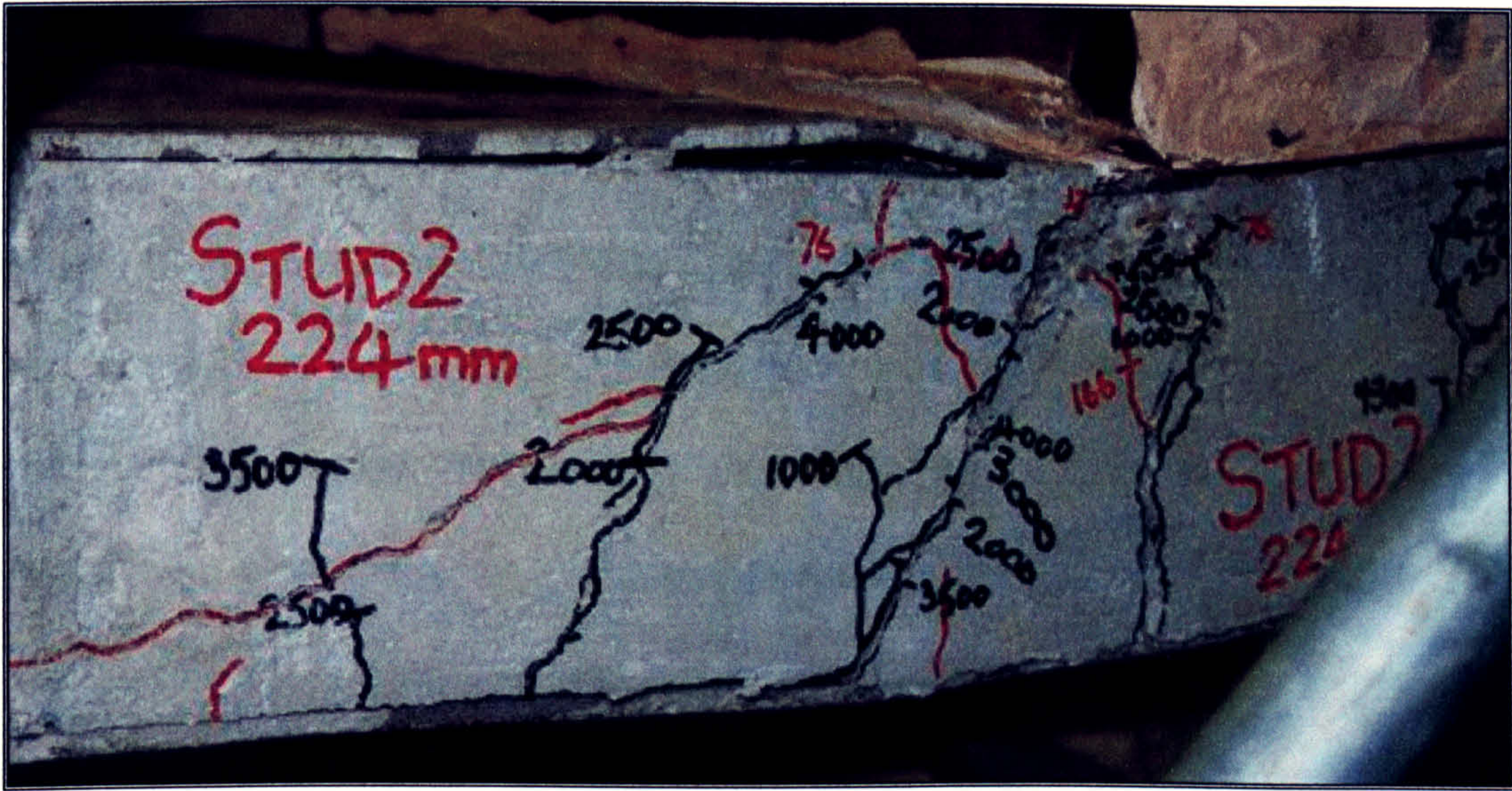
Plate 4.1. Failure of test specimen Stud2
