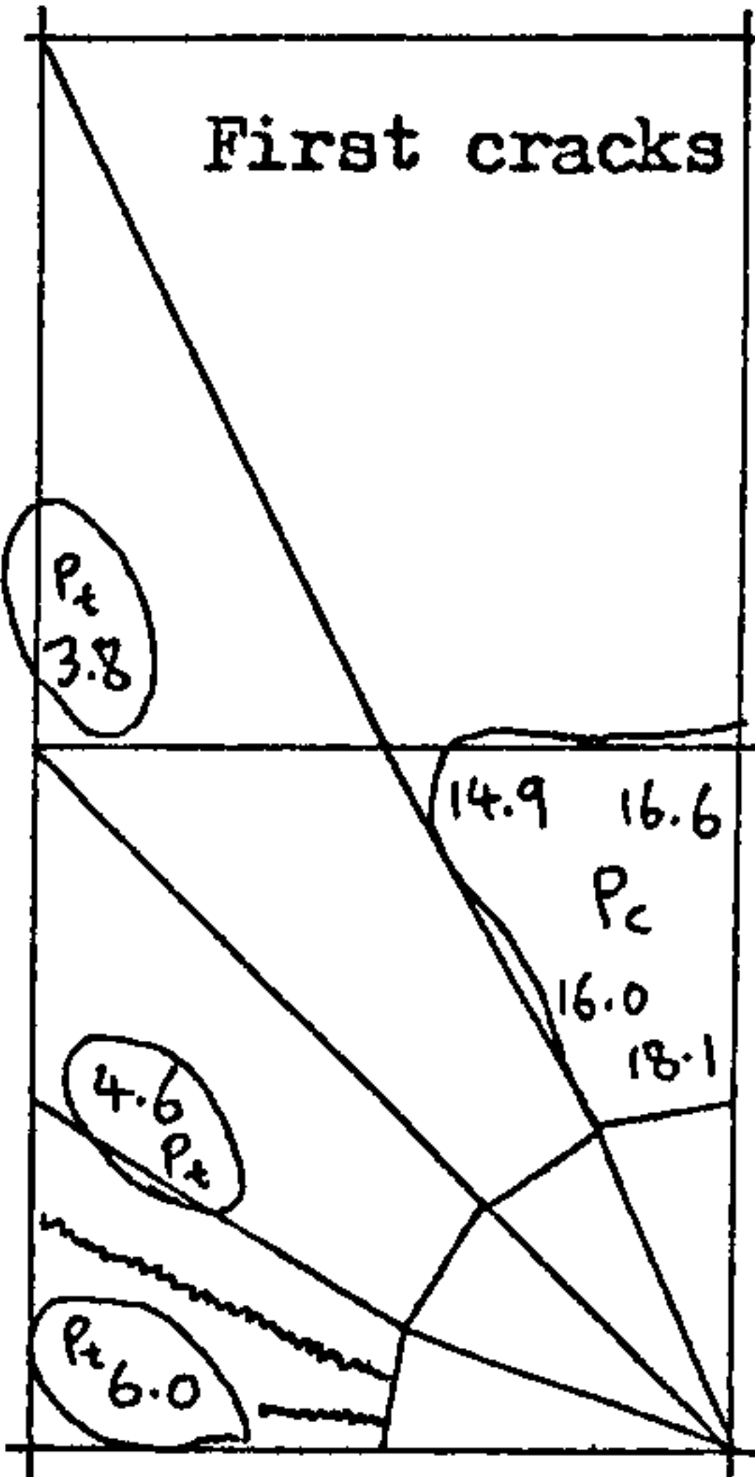
Load step 18
