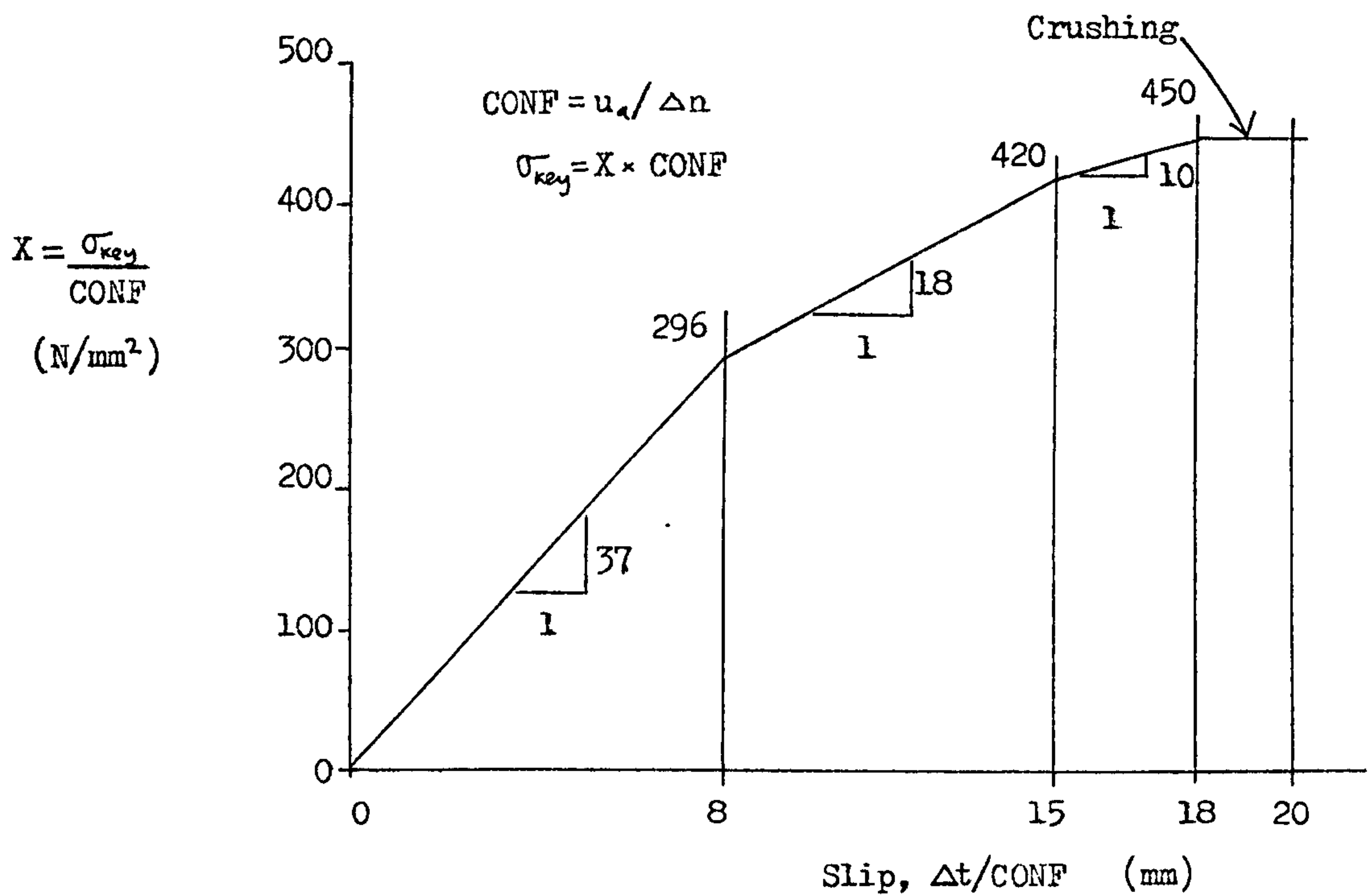
FIGURE 5.6 TYPICAL LOAD-SLIP CURVE FOR A CONNECTION WITH SHEAR KEYS.
