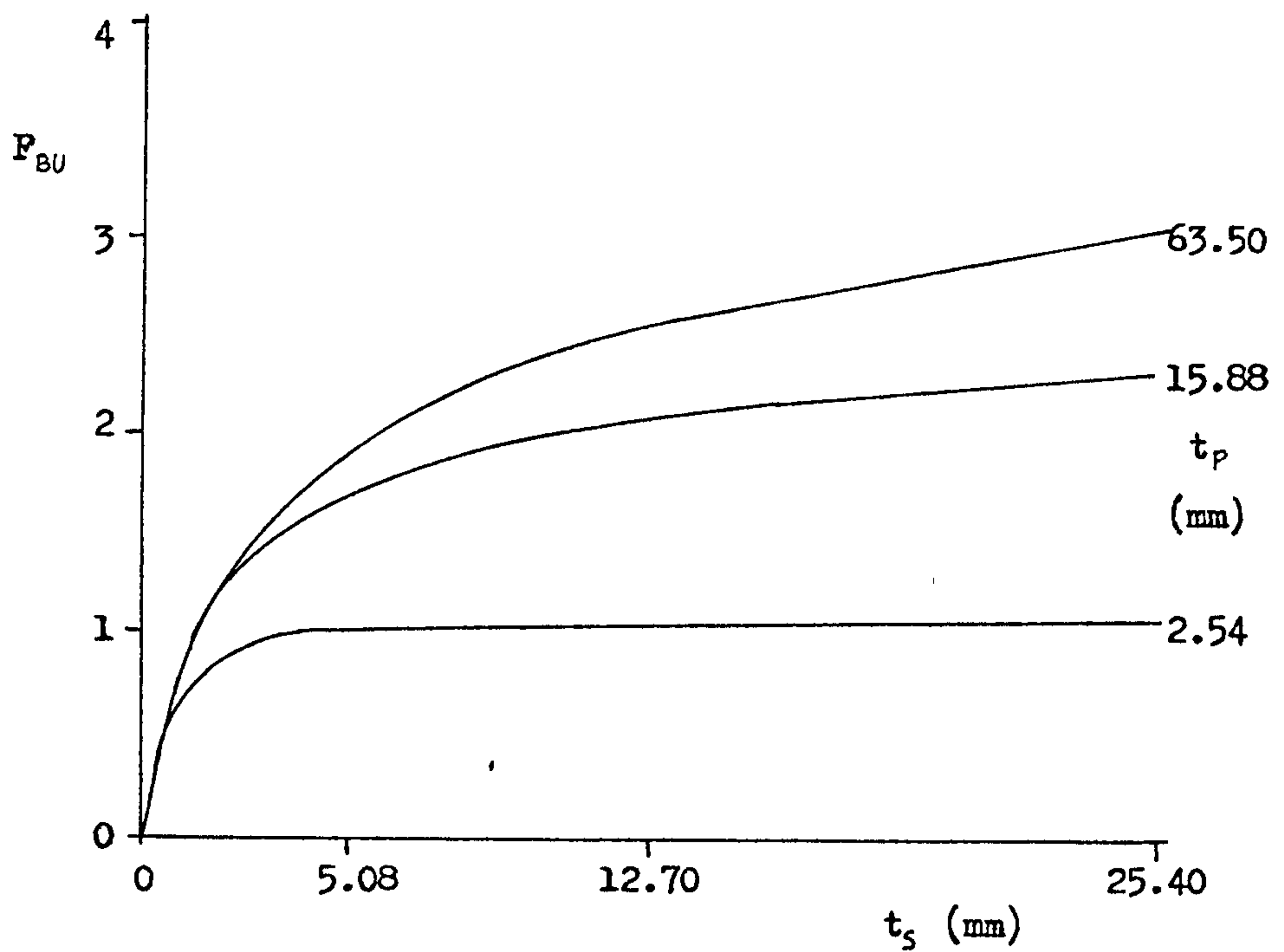
(b) New Bond Strength Formula Predictions
