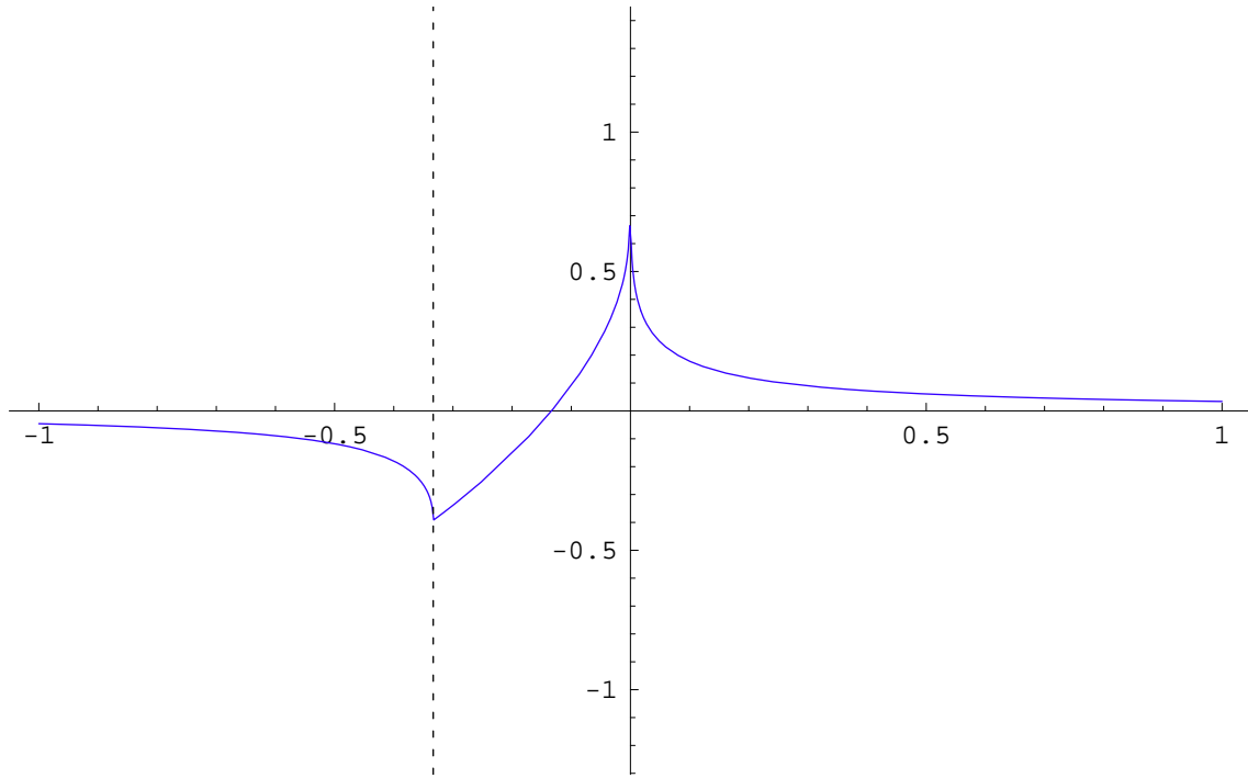
Figure 1: A_{ee} as a function of \lambda . The dashed line is at \lambda = -1/3 .
