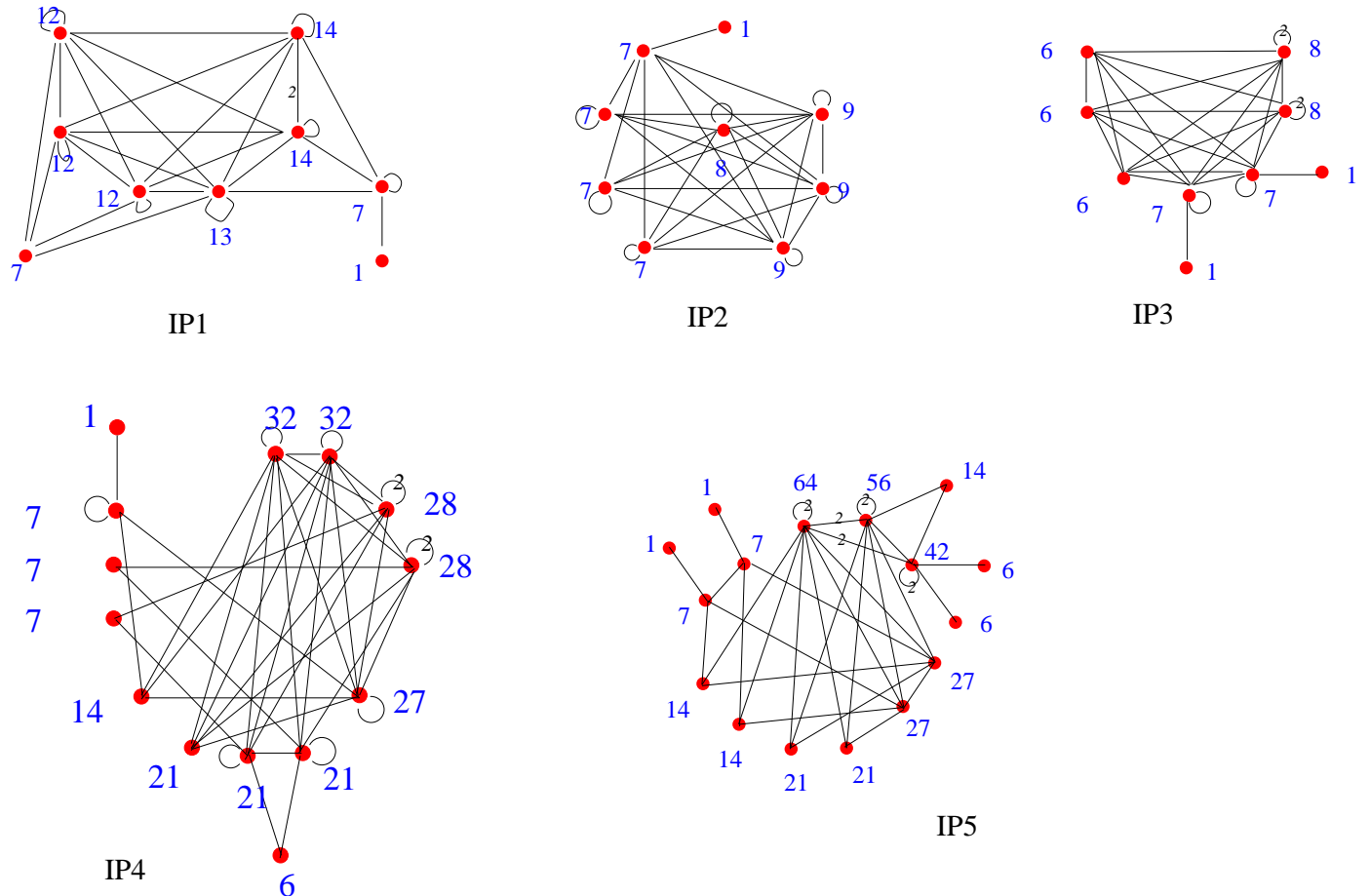
Figure 2: The quiver diagram with respect to the fundamental 7 for the 5 irreducible primitive discrete subgroups of G_2 .
