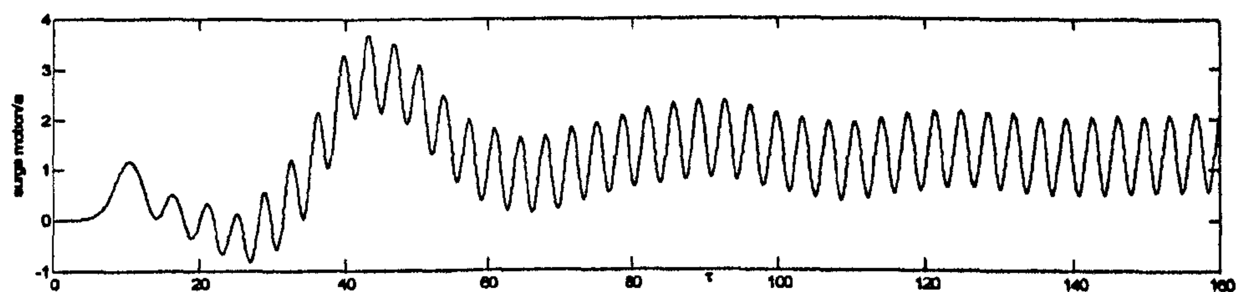
Fig.9.4.7 (a) Surge
