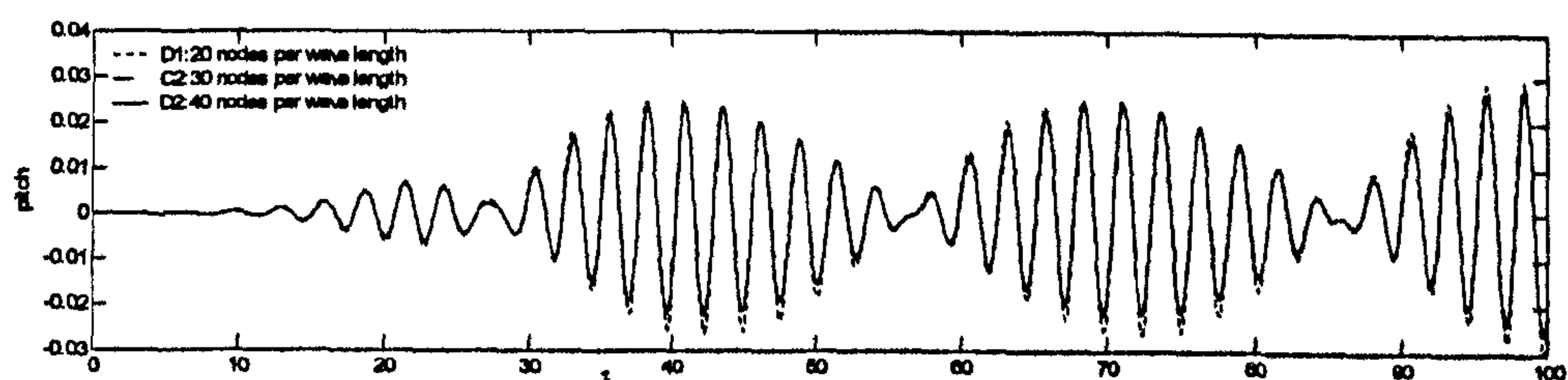
Fig.9.2.2 Pitch histories in cases with different mesh sizes
