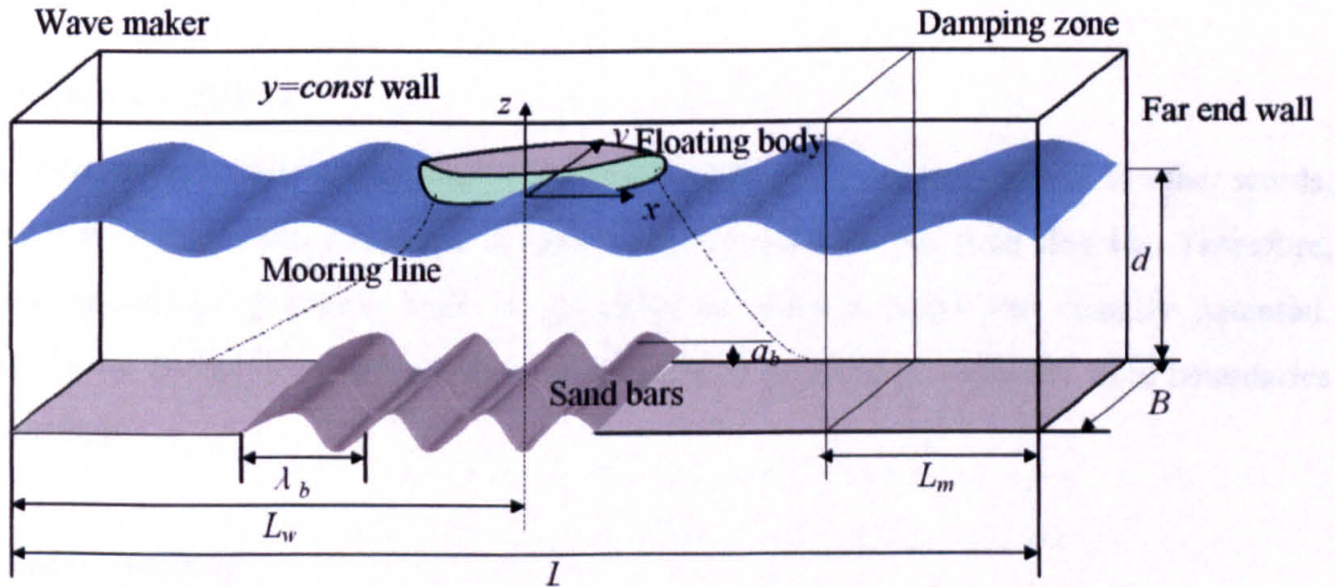
Fig. 3.0.1 Sketch of the fluid domain
