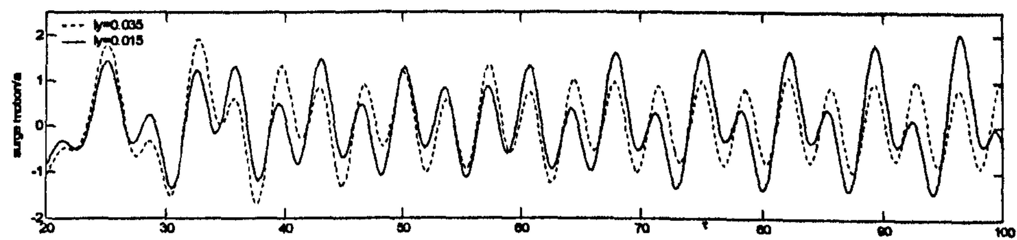
Fig. 9.4.6 (a) surge
