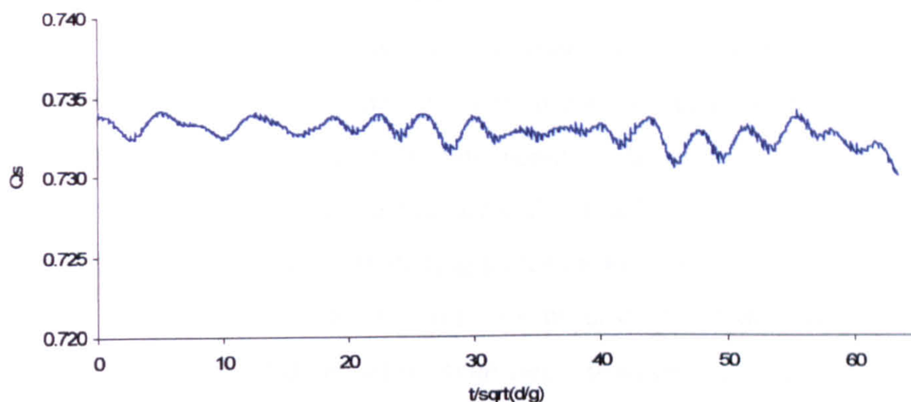
Fig.9.5.3 Mesh quality during the calculation in Case 2 ( \omega = 1.7691 , \alpha=0.025 , Wigley Hull with L_b=1.0, B_b=0.2, D_r=0.15 )
