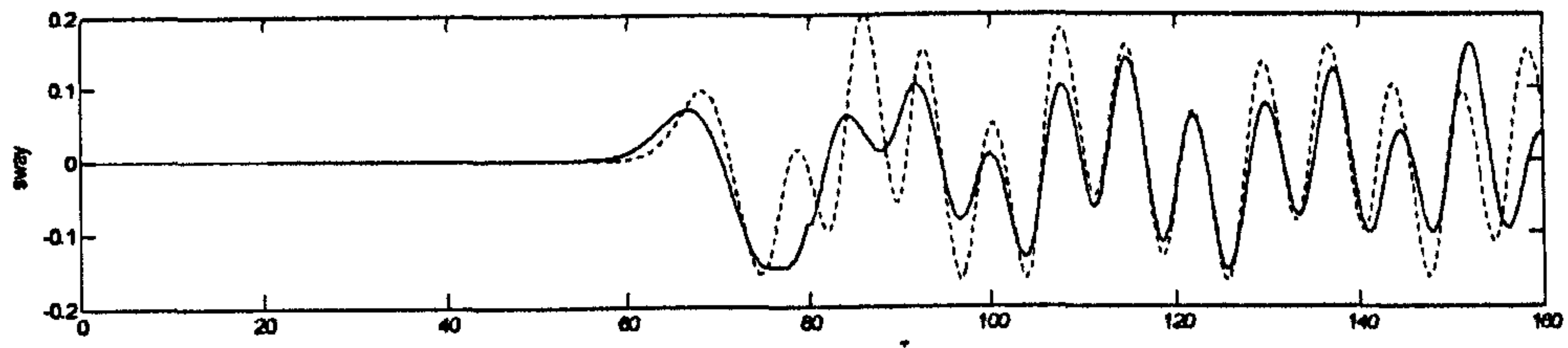
Fig.8.2.24 (a) sway
