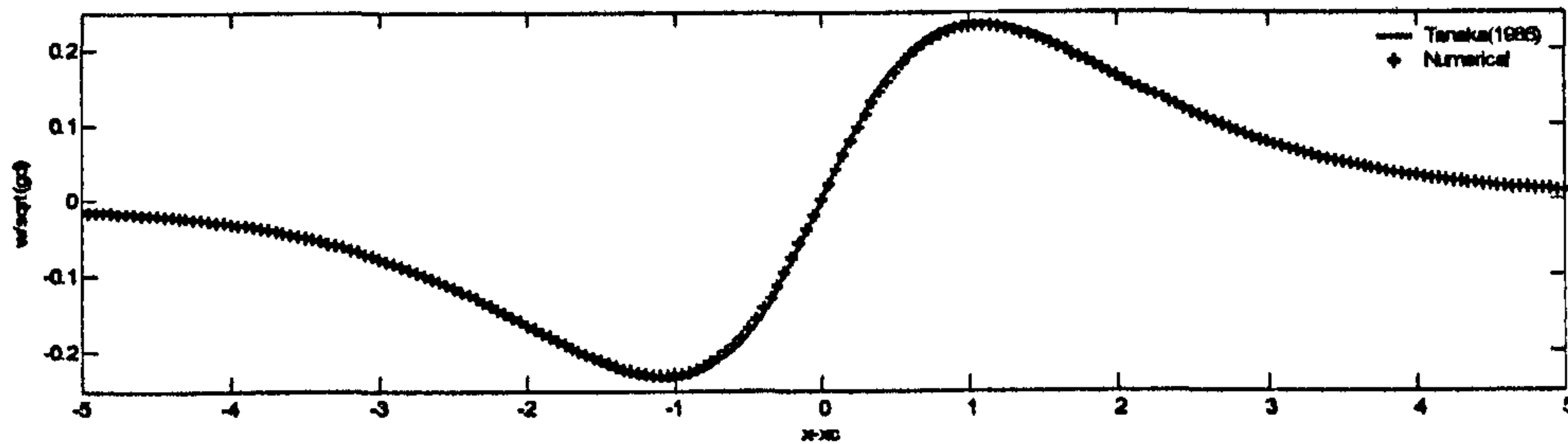
Fig.5.3.5 (b) Vertical velocity component ( y=0 )
