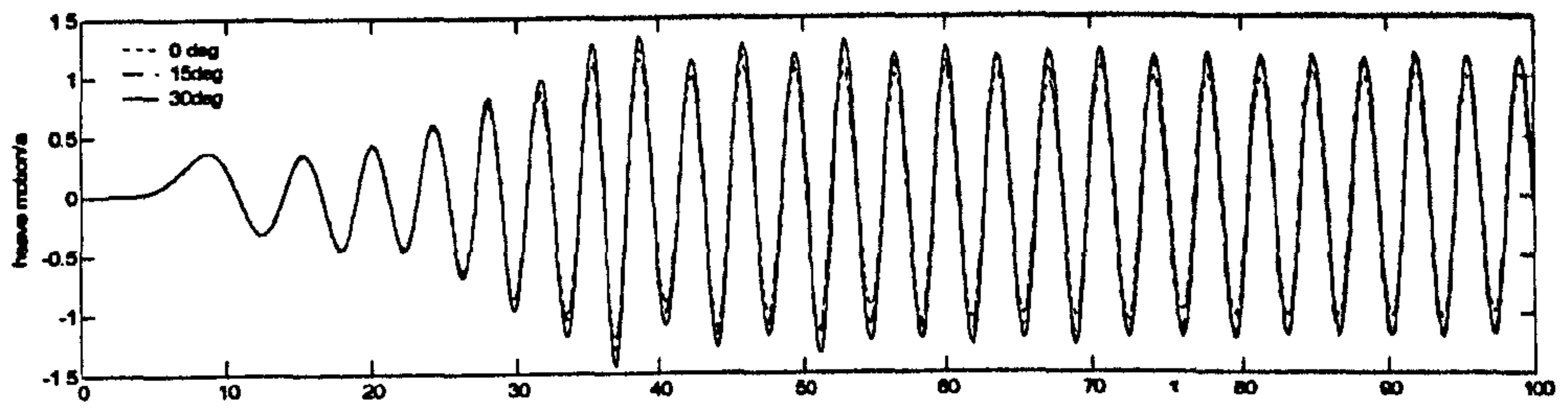
Fig.9.4. 11 (b) heave
