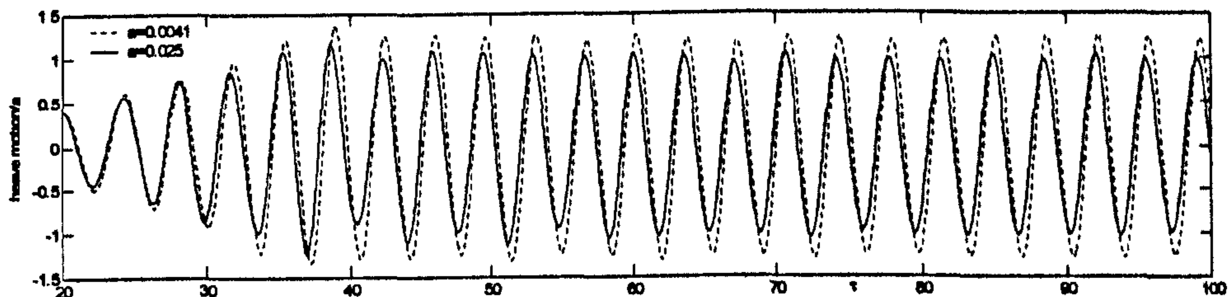
Fig.9.4.3 (b) heave
