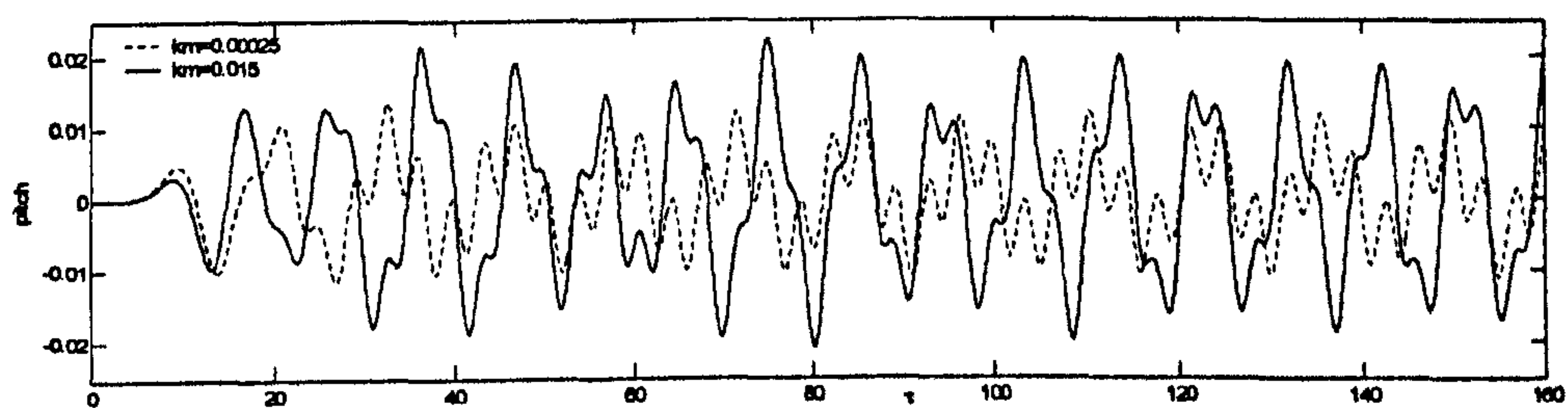
Fig. 9.4.9 (b) pitch
