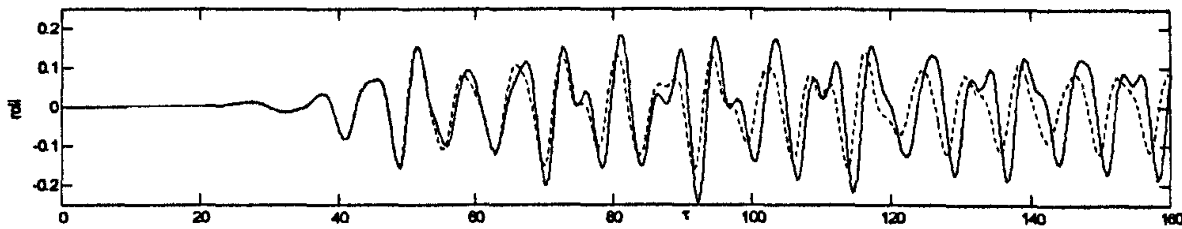
Fig.8.2.22 (c) roll
