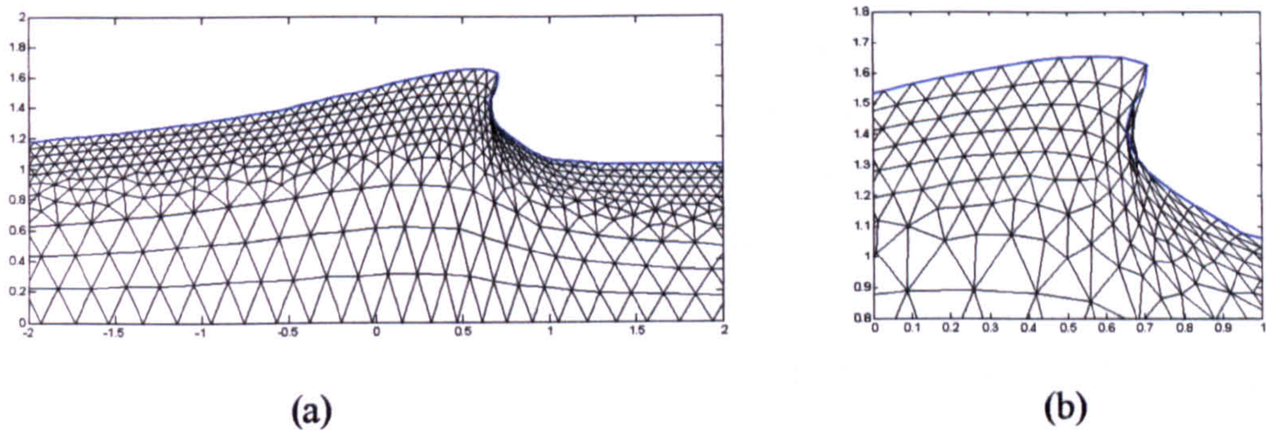
Fig.4.2.9 2D mesh on the vertical wall in the case with an assumed overturning wave (\gamma_f=1.7, \kappa=0) ( Thick curve: free surface)
