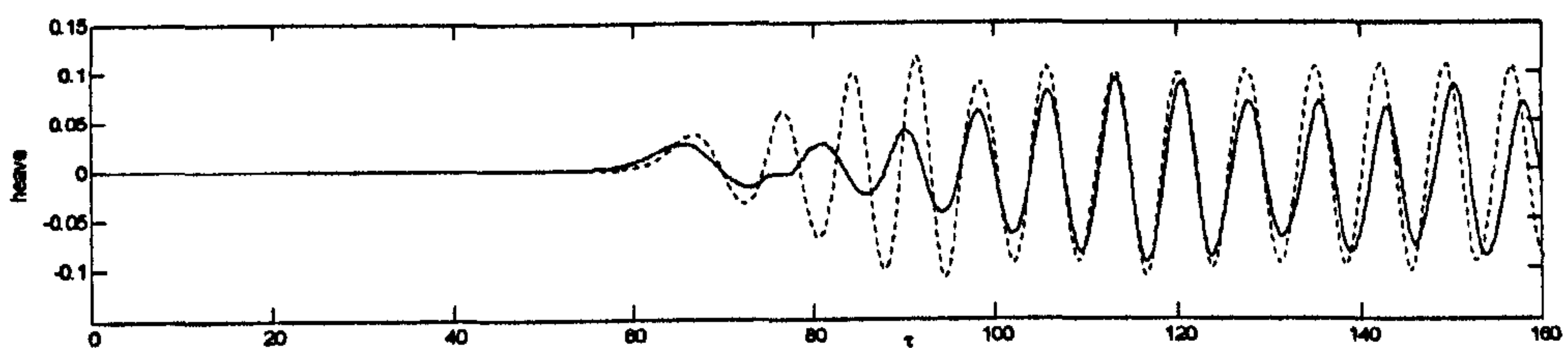
Fig.8.2.24 (b) heave
