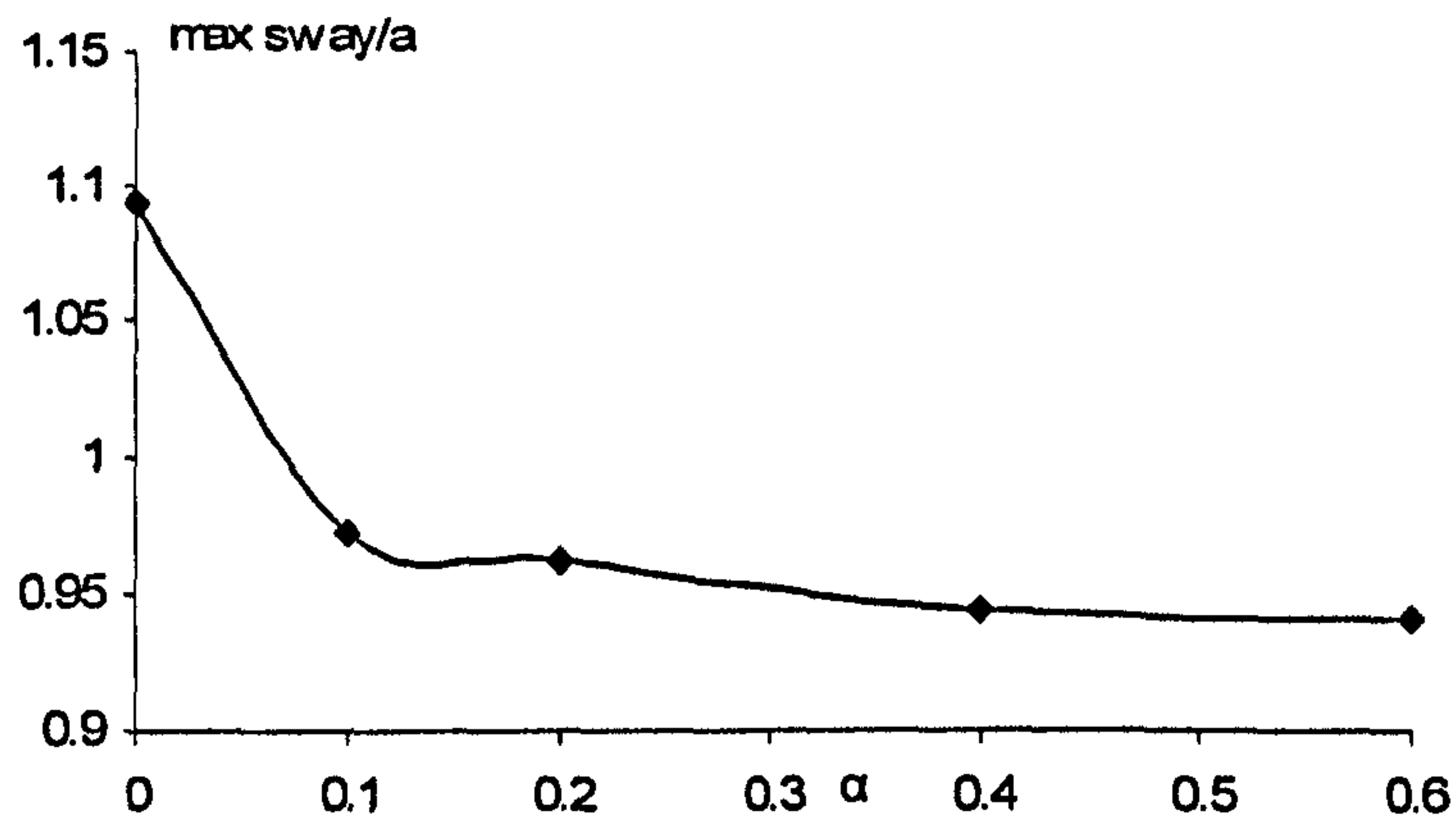
Fig.8.2.3 Maximum displacement in cases with different \alpha (\varpi = 0.25 \text{ and } T_d = L_w / C_g)
