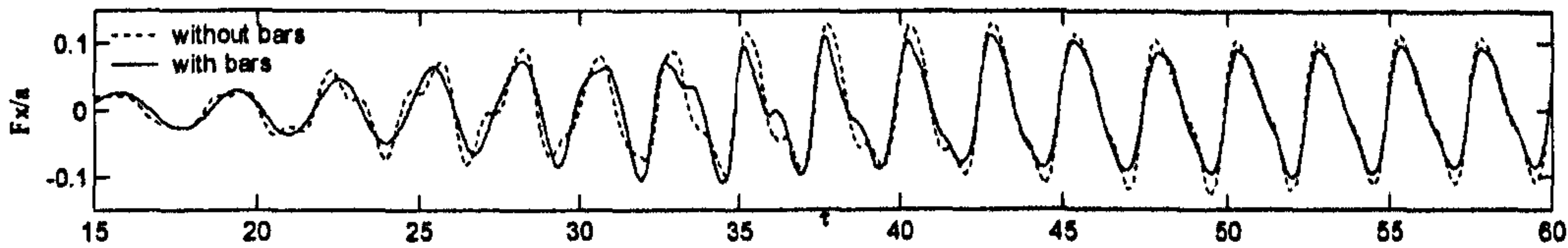
Fig.8.2.20 Comparison of sway forces acting on the floating body with and without sandbars ( \xi = 0.65 , the wave height is about 7cm)
