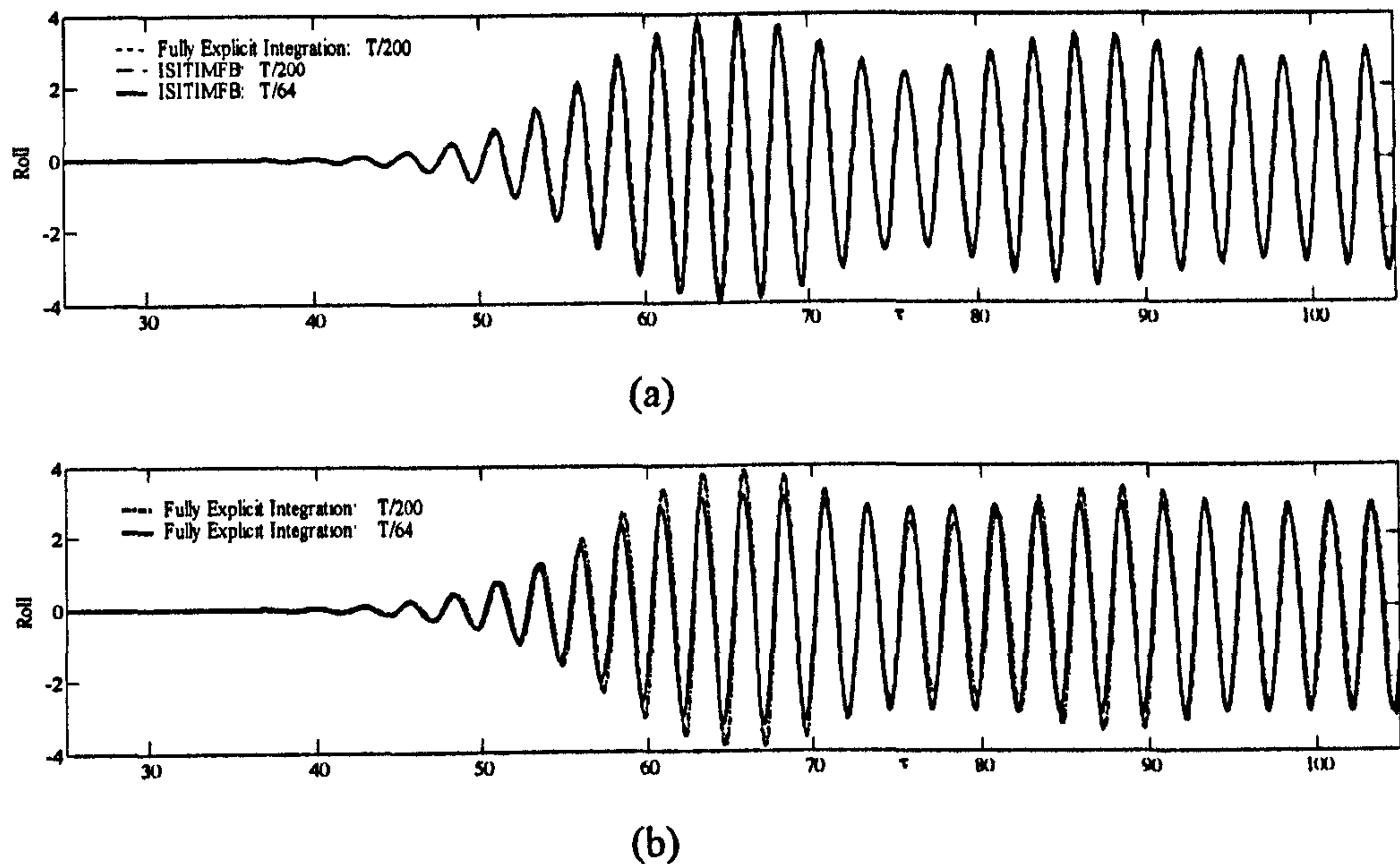
Fig.8.2.8 Comparison of roll motions from the ISITIMFB and explicit procedures
