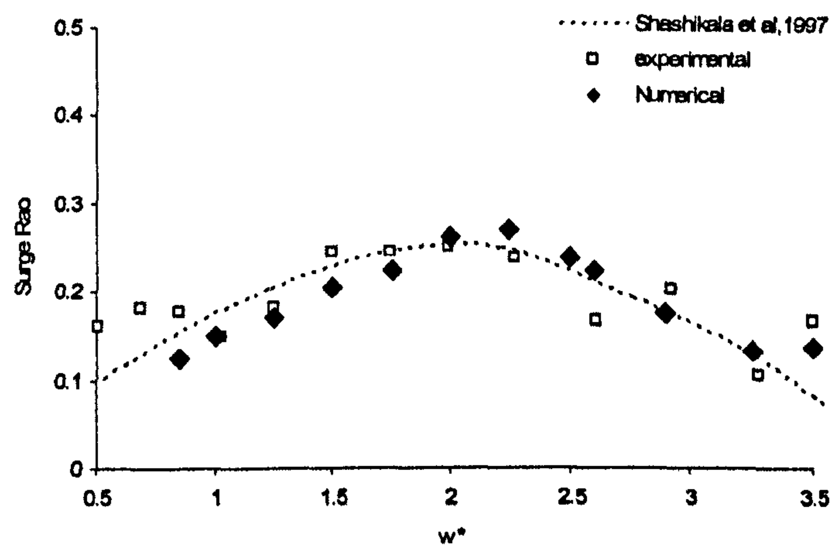
Fig.9.3.2 (a) Surge RAO
