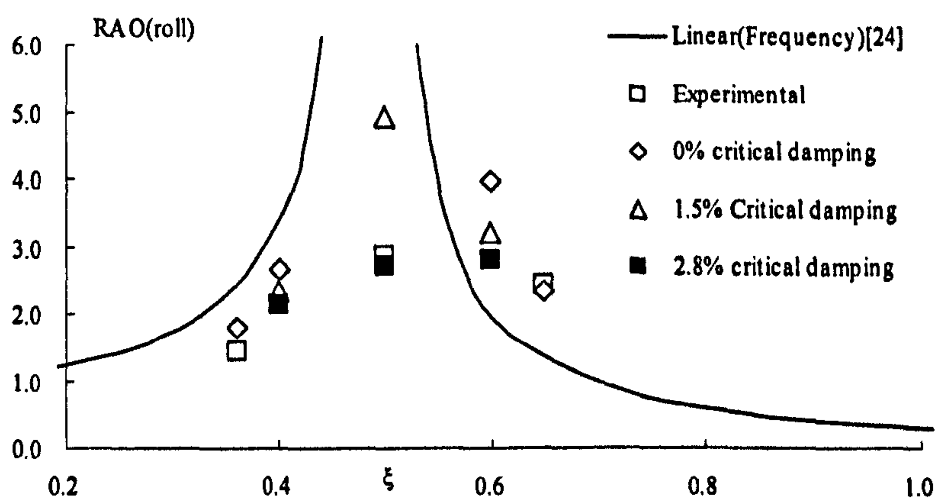
Fig. 8.2.11 RAO of roll motion in cases with roll artificial damping
