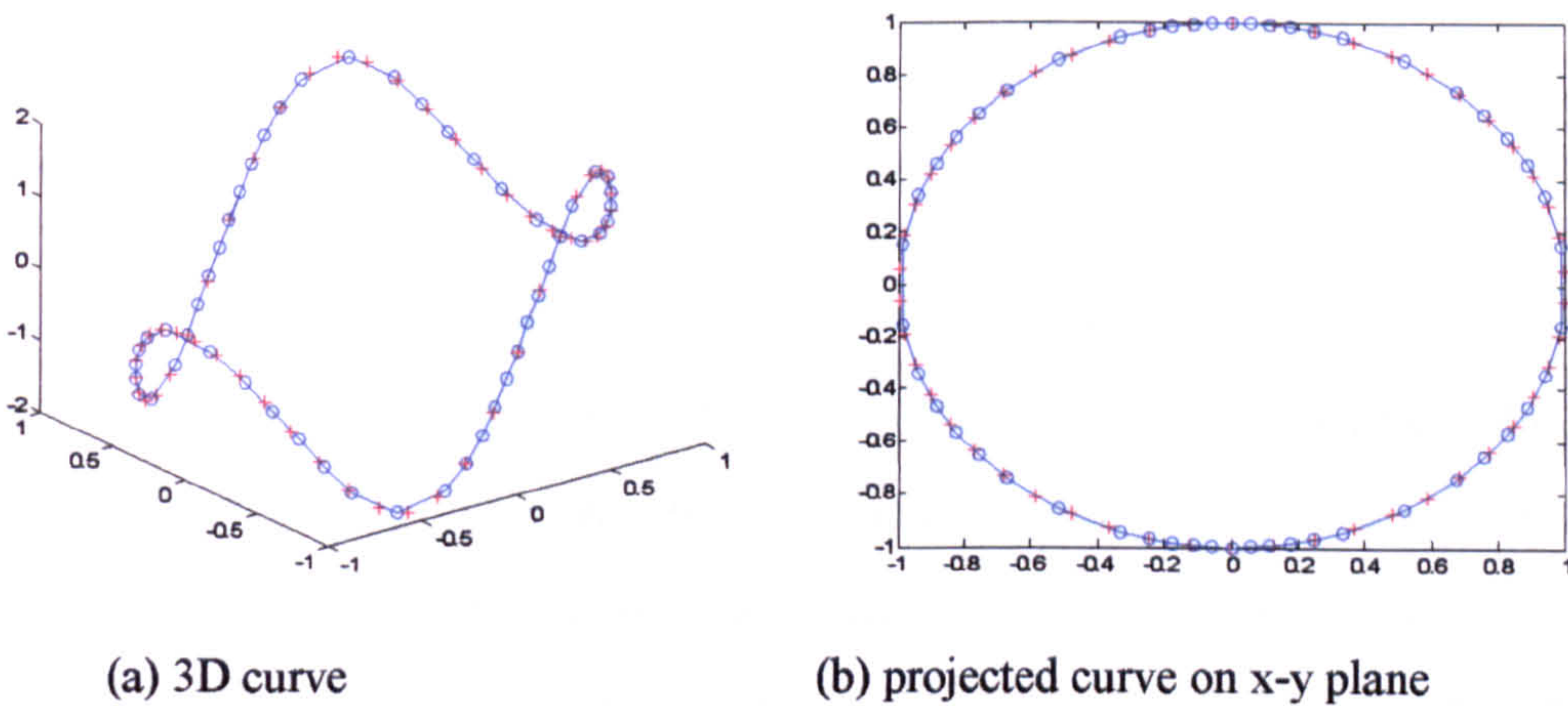
Fig.4.4.2 Initial nodes and those after being redistributed on a 3D curve (‘+’: before redistributed; ‘o’: after redistributed)
