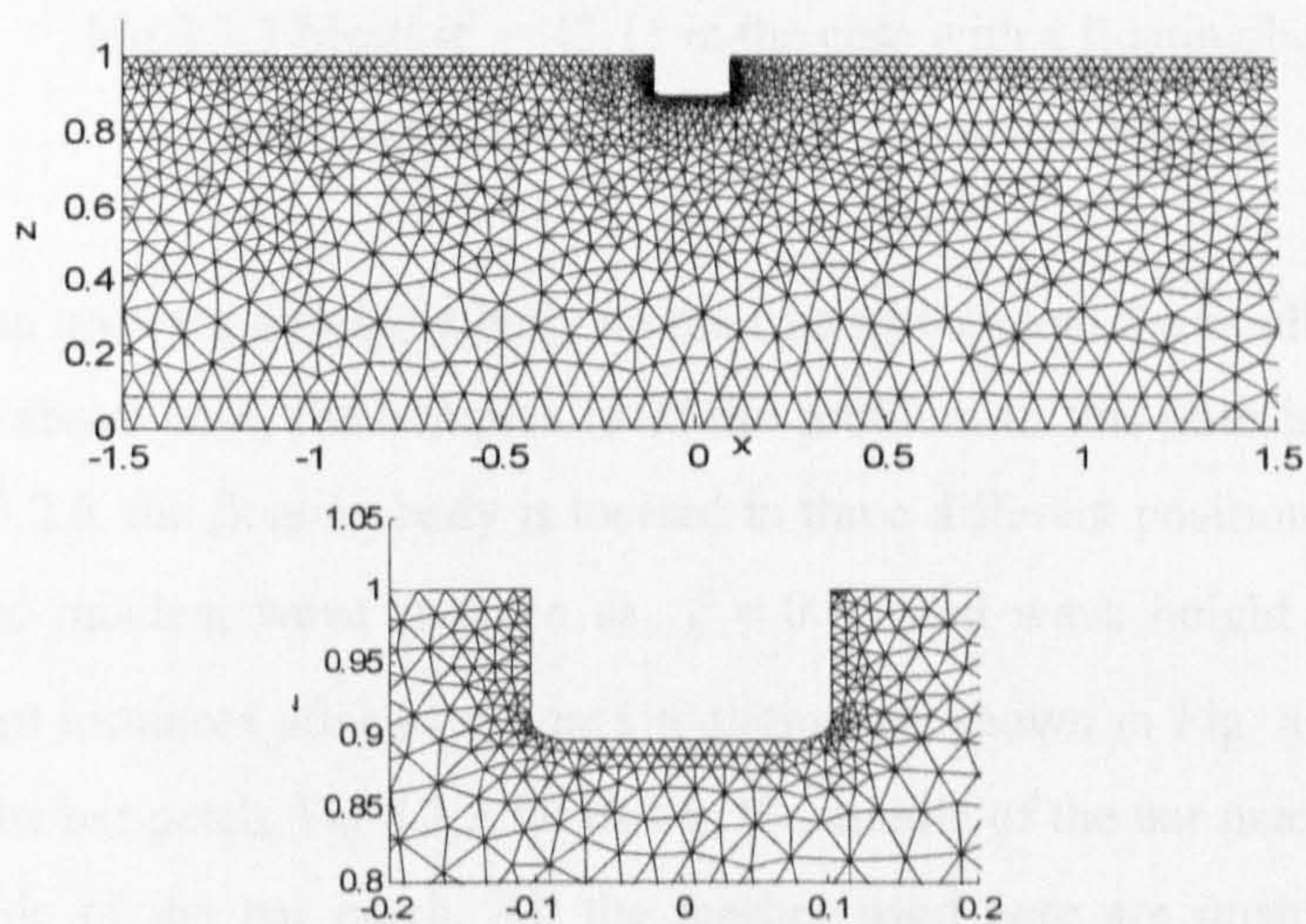
Fig.8.3.1 Initial mesh in the case with a floating body
