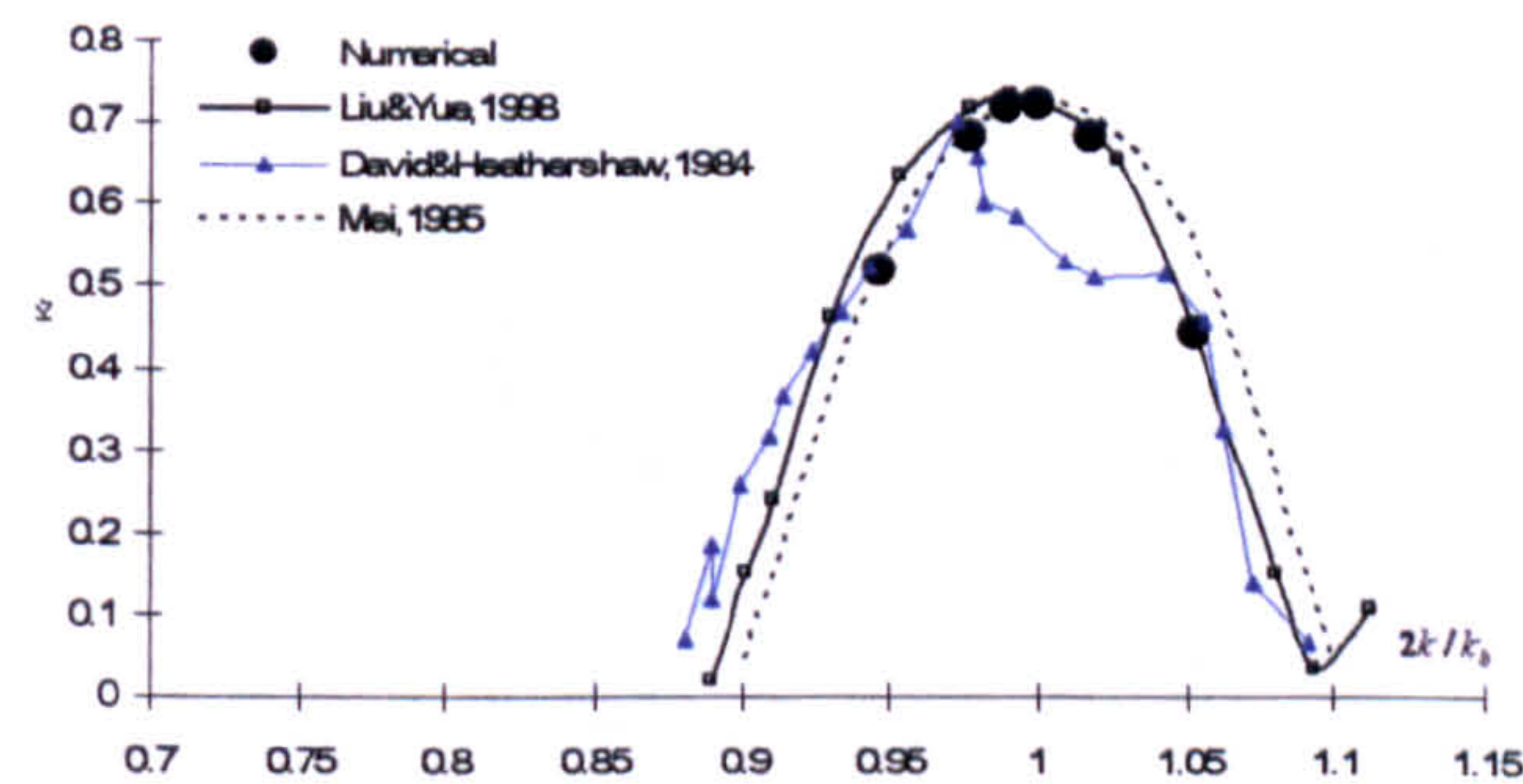
(b) Ten bars, a_b/d = 0.16
