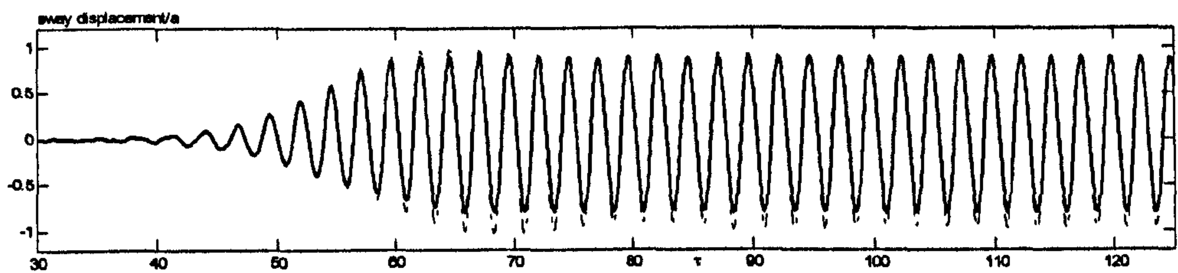
Fig.8.2.13 (a)sway
