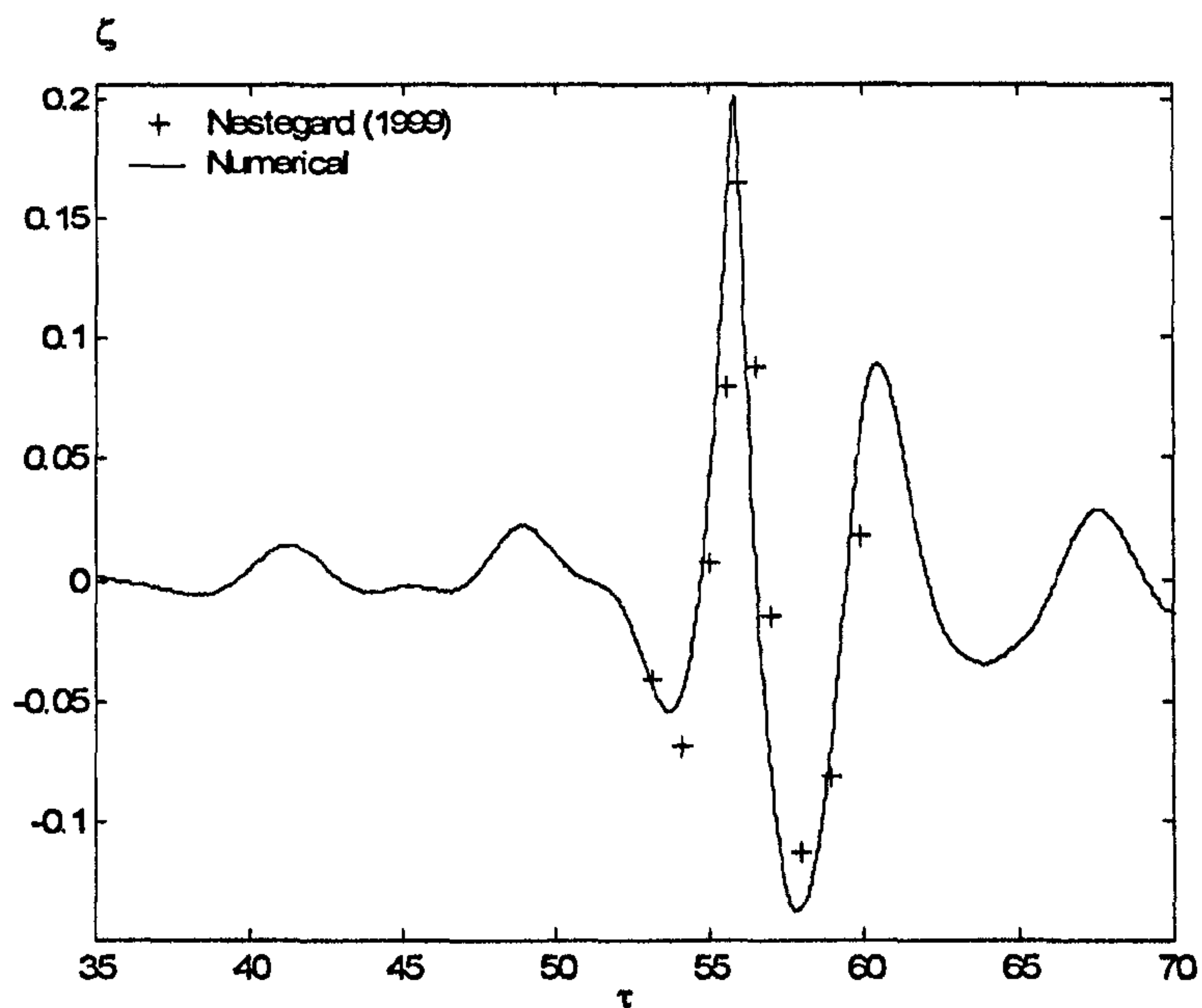
Fig.7.1.7 (a) ( \alpha_{\text{random}} = 0.612 )
