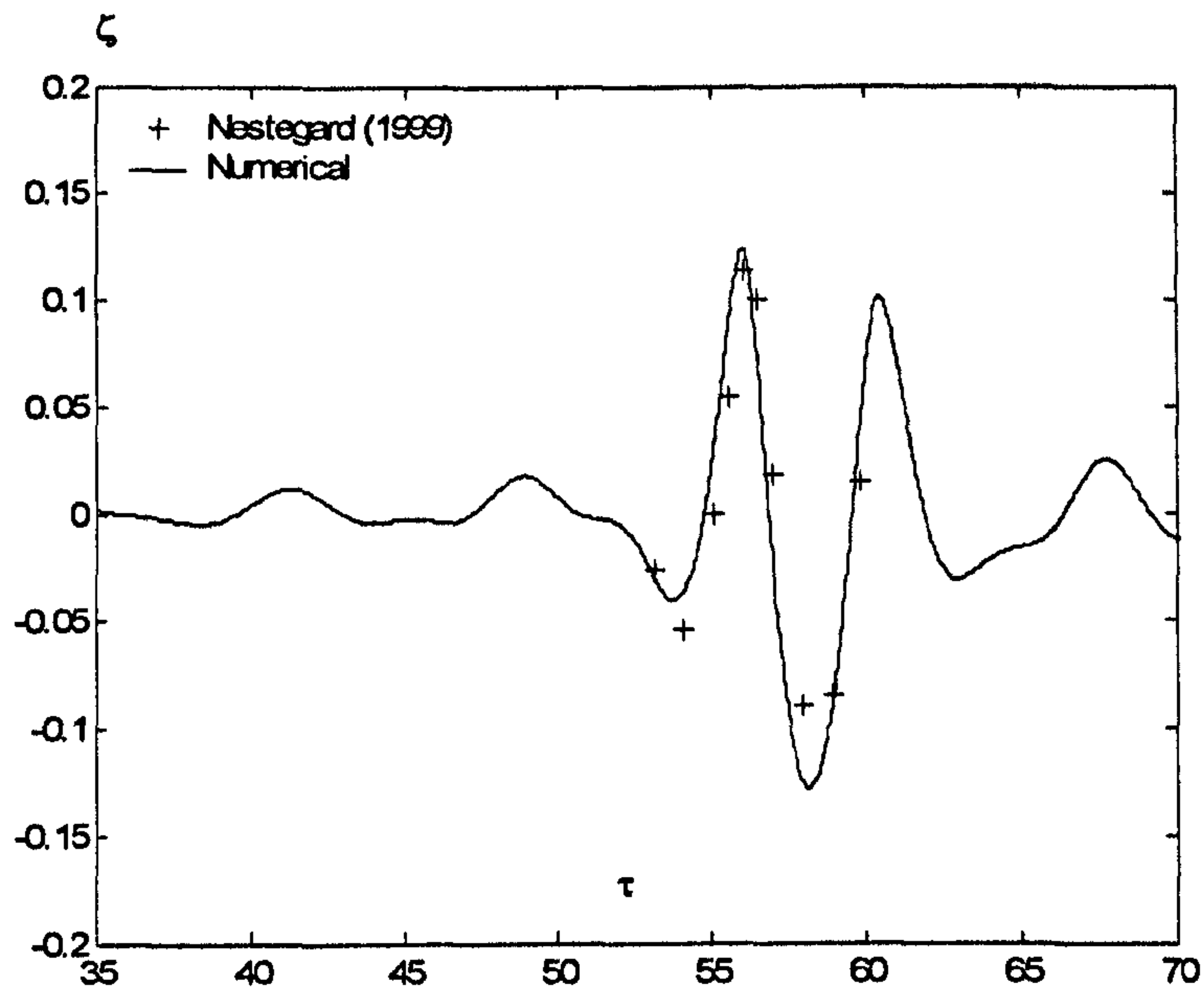
Fig.7.1.7 (a) ( \alpha_{\text{random}} = 0.612 )
