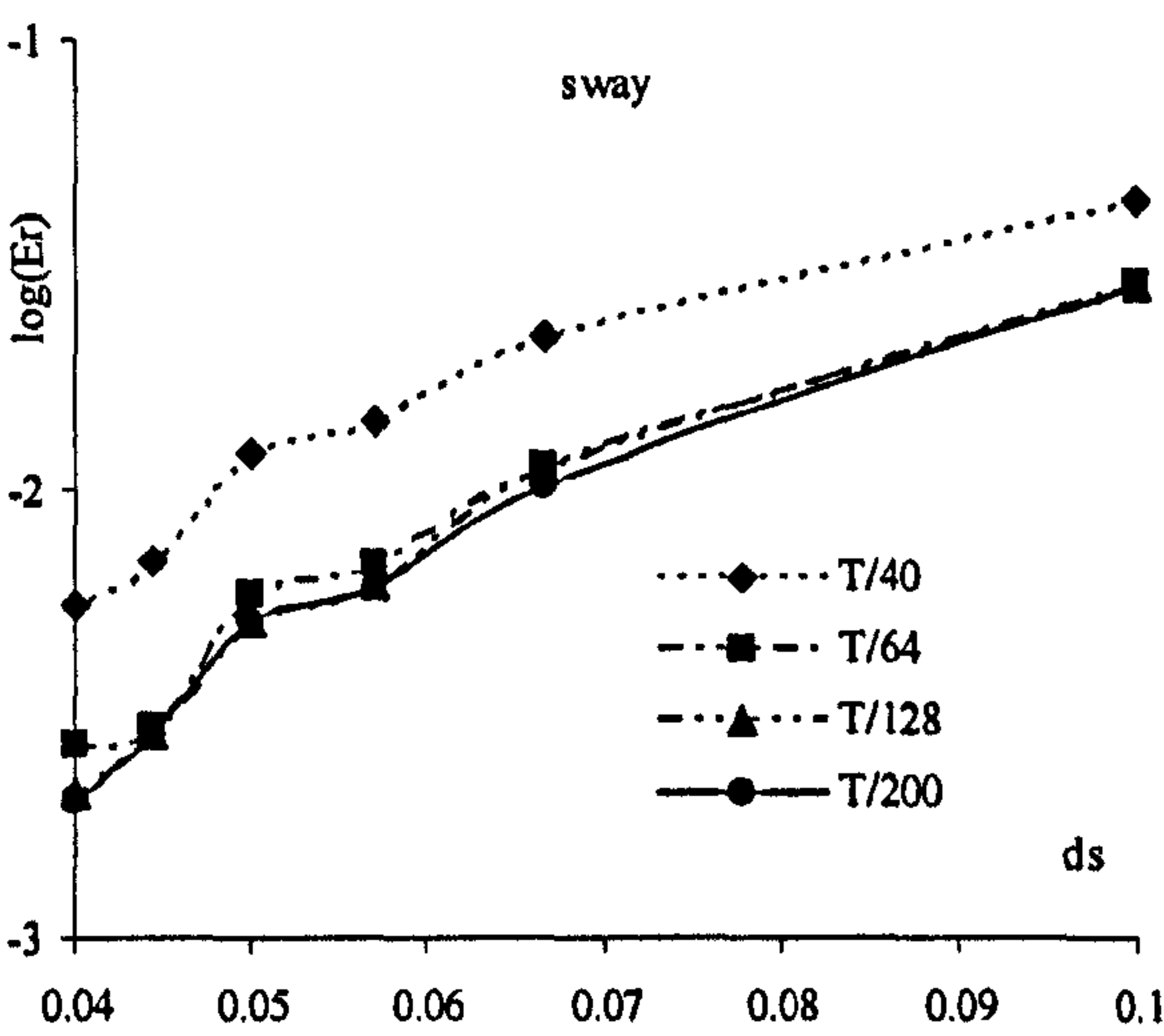
(a) Sway
