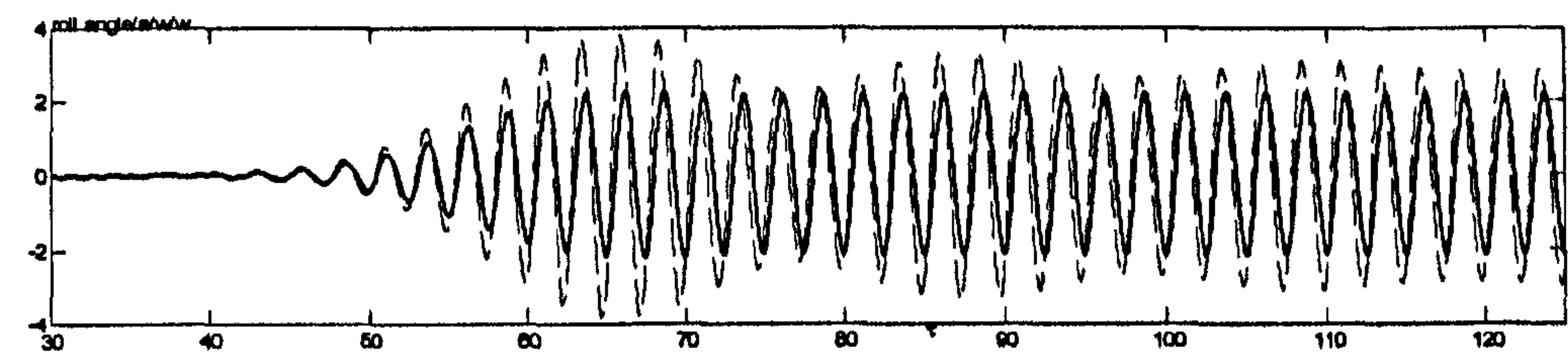
Fig.8.2.13(c) roll
