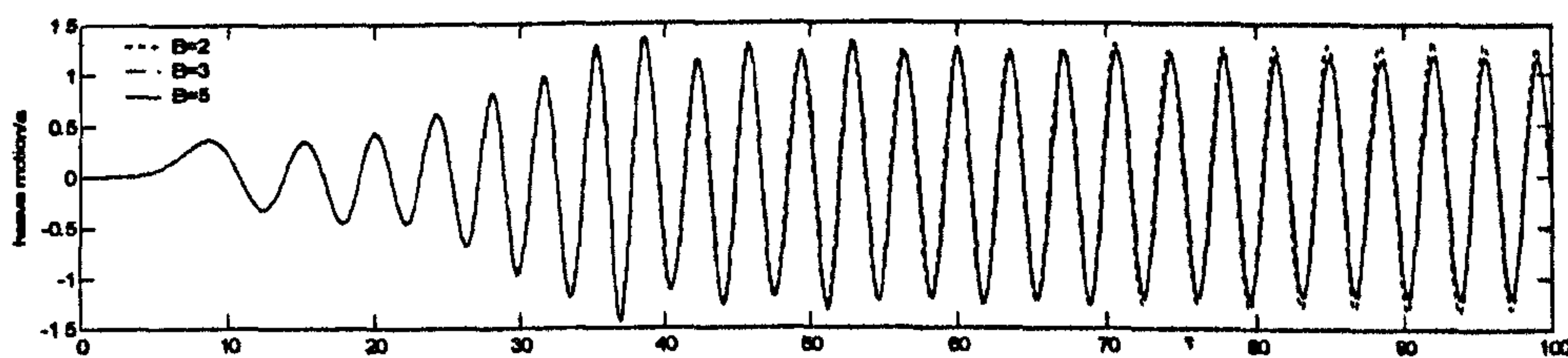
Fig. 9.4.10 (c) heave
