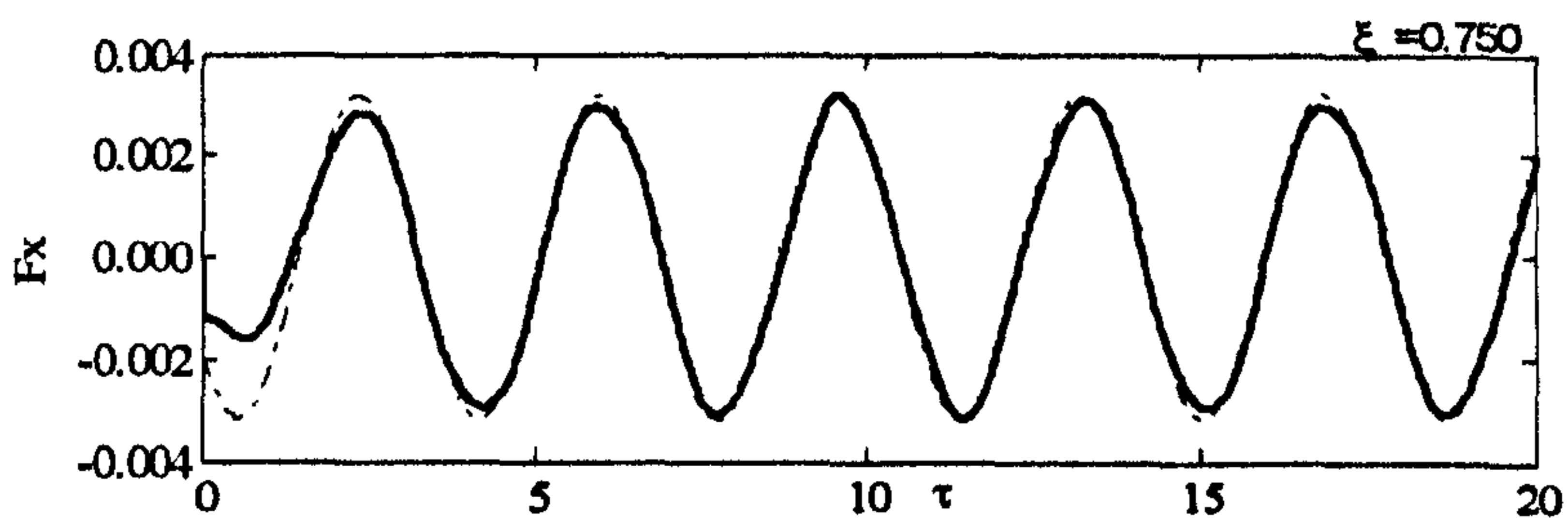
Fig.8.1.2 (c) forced sway \xi = 0.750
